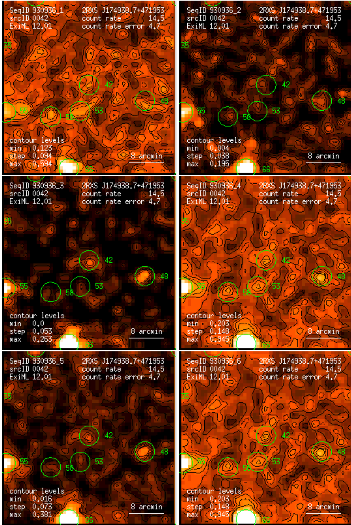
Figure 42: RASS 930936: detection 0042: band rate images, Gaussian filter: (1) PSPC channels 11 – 41, (2) 52 – 90, (3) 91 – 201, (4) 11 – 235, (5) 52 – 201, (6) 11 – 201. Broad band rates in counts/ks. Band rate contour levels in counts/ks/arcmin 2 .
