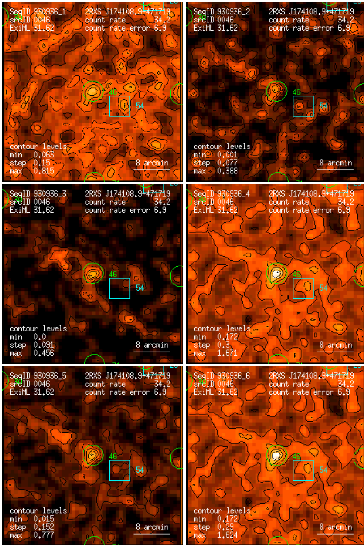
Figure 46: RASS 930936: detection 0046: band rate images, Gaussian filter: (1) PSPC channels 11 – 41, (2) 52 – 90, (3) 91 – 201, (4) 11 – 235, (5) 52 – 201, (6) 11 – 201. Broad band rates in counts/ks. Band rate contour levels in counts/ks/arcmin 2 .
