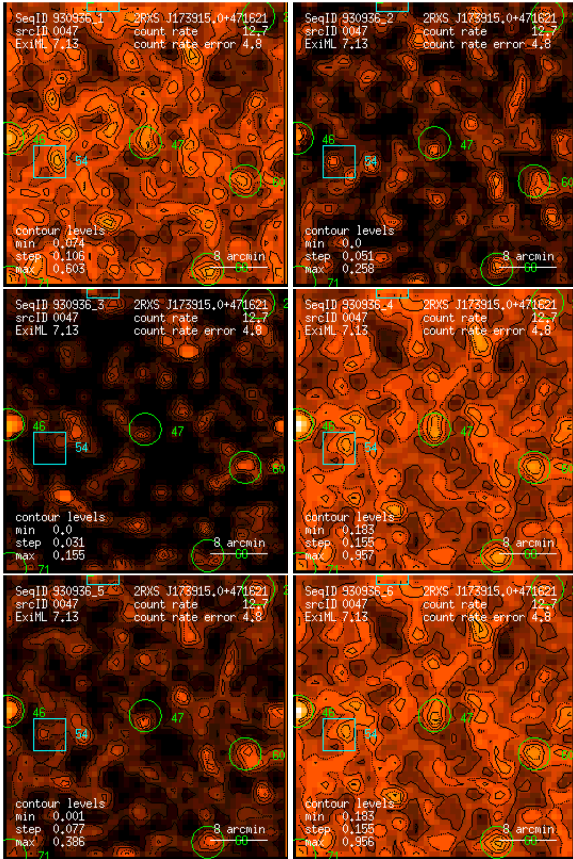
Figure 47: RASS 930936: detection 0047: band rate images, Gaussian filter: (1) PSPC channels 11 – 41, (2) 52 – 90, (3) 91 – 201, (4) 11 – 235, (5) 52 – 201, (6) 11 – 201. Broad band rates in counts/ks. Band rate contour levels in counts/ks/arcmin 2 .
