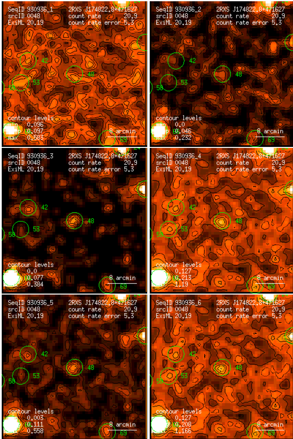
Figure 48: RASS 930936: detection 0048: band rate images, Gaussian filter: (1) PSPC channels 11 – 41, (2) 52 – 90, (3) 91 – 201, (4) 11 – 235, (5) 52 – 201, (6) 11 – 201. Broad band rates in counts/ks. Band rate contour levels in counts/ks/arcmin 2 .
