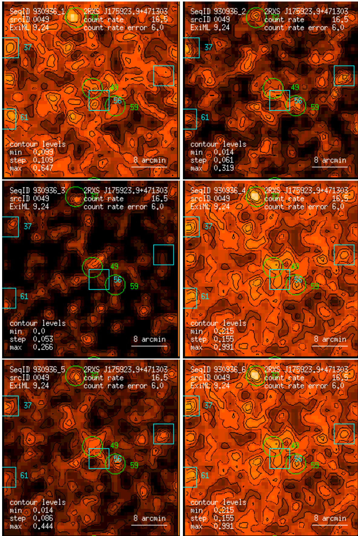
Figure 49: RASS 930936: detection 0049: band rate images, Gaussian filter: (1) PSPC channels 11 – 41, (2) 52 – 90, (3) 91 – 201, (4) 11 – 235, (5) 52 – 201, (6) 11 – 201. Broad band rates in counts/ks. Band rate contour levels in counts/ks/arcmin 2 .
