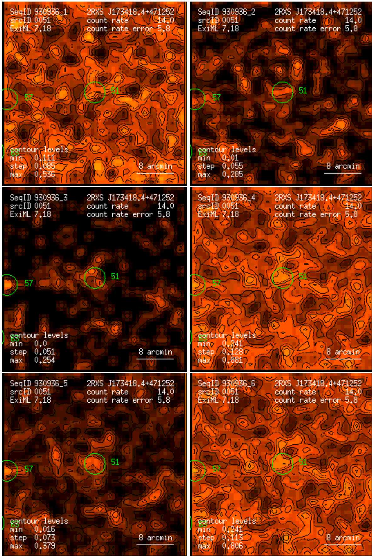
Figure 51: RASS 930936: detection 0051: band rate images, Gaussian filter: (1) PSPC channels 11 – 41, (2) 52 – 90, (3) 91 – 201, (4) 11 – 235, (5) 52 – 201, (6) 11 – 201. Broad band rates in counts/ks. Band rate contour levels in counts/ks/arcmin 2 .
