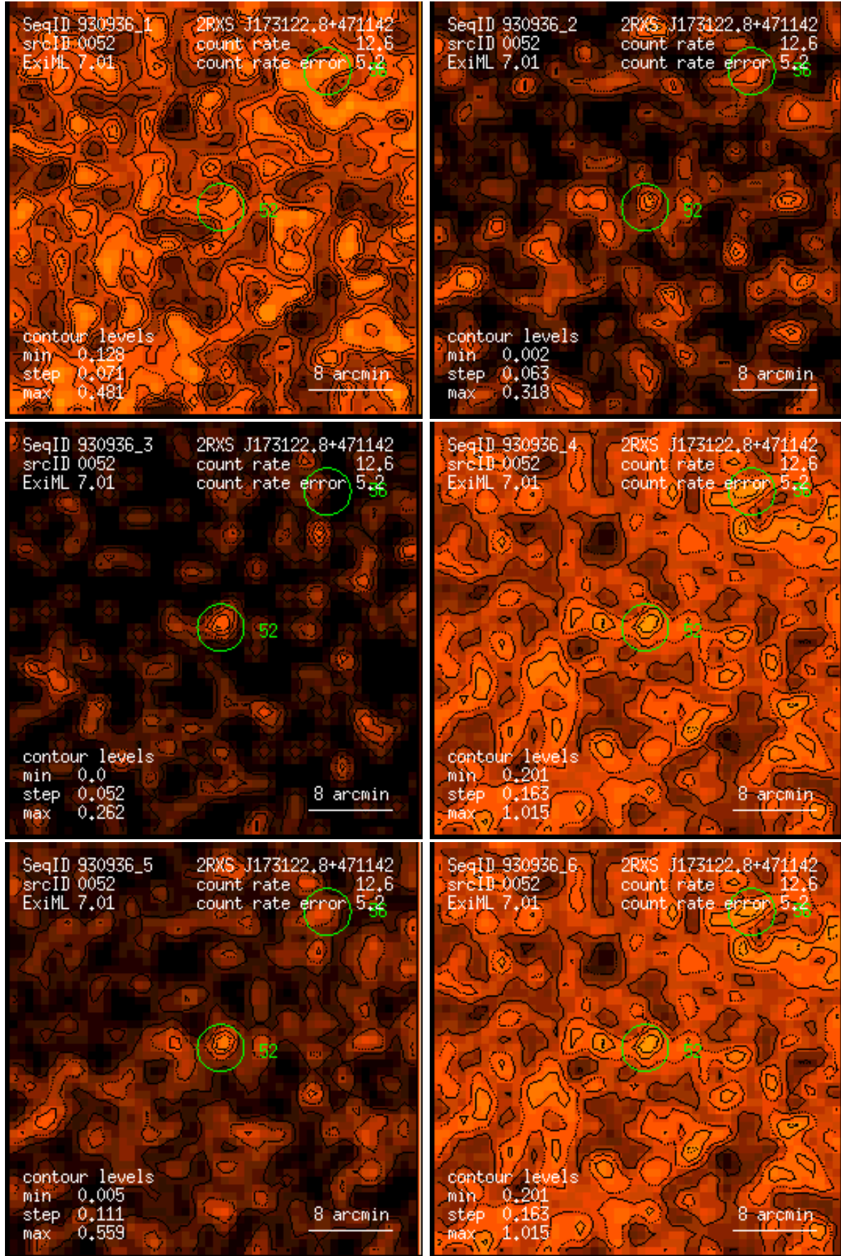
Figure 52: RASS 930936: detection 0052: band rate images, Gaussian filter: (1) PSPC channels 11 – 41, (2) 52 – 90, (3) 91 – 201, (4) 11 – 235, (5) 52 – 201, (6) 11 – 201. Broad band rates in counts/ks. Band rate contour levels in counts/ks/arcmin 2 .
