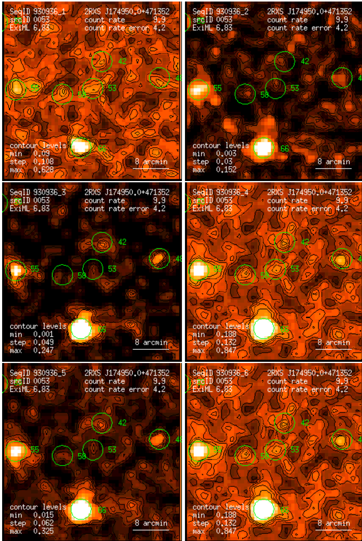
Figure 53: RASS 930936: detection 0053: band rate images, Gaussian filter: (1) PSPC channels 11 – 41, (2) 52 – 90, (3) 91 – 201, (4) 11 – 235, (5) 52 – 201, (6) 11 – 201. Broad band rates in counts/ks. Band rate contour levels in counts/ks/arcmin 2 .
