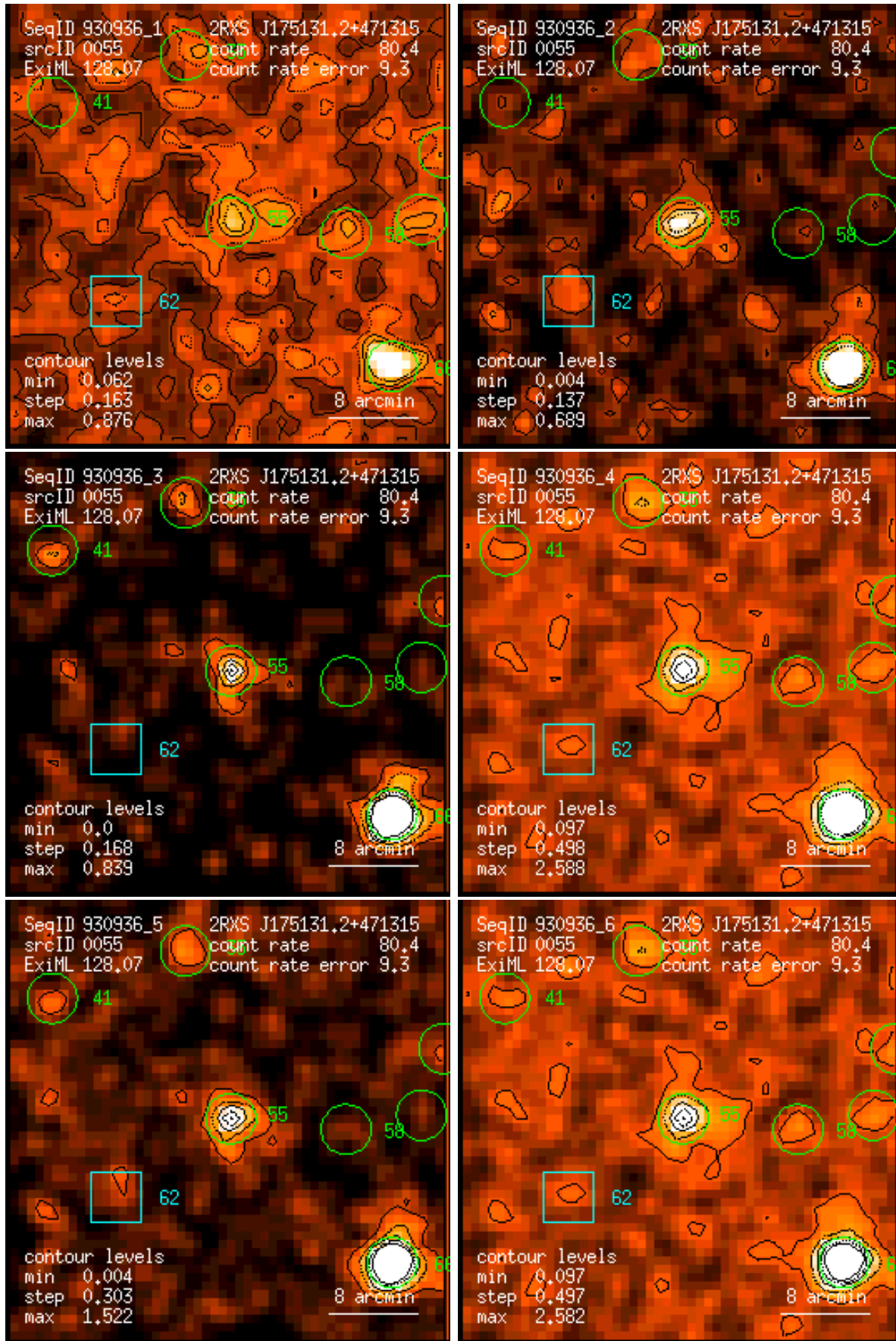
Figure 55: RASS 930936: detection 0055: band rate images, Gaussian filter: (1) PSPC channels 11 – 41, (2) 52 – 90, (3) 91 – 201, (4) 11 – 235, (5) 52 – 201, (6) 11 – 201. Broad band rates in counts/ks. Band rate contour levels in counts/ks/arcmin 2 .
