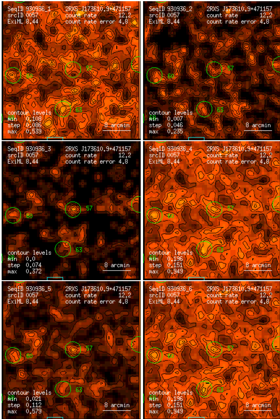
Figure 57: RASS 930936: detection 0057: band rate images, Gaussian filter: (1) PSPC channels 11 – 41, (2) 52 – 90, (3) 91 – 201, (4) 11 – 235, (5) 52 – 201, (6) 11 – 201. Broad band rates in counts/ks. Band rate contour levels in counts/ks/arcmin 2 .
