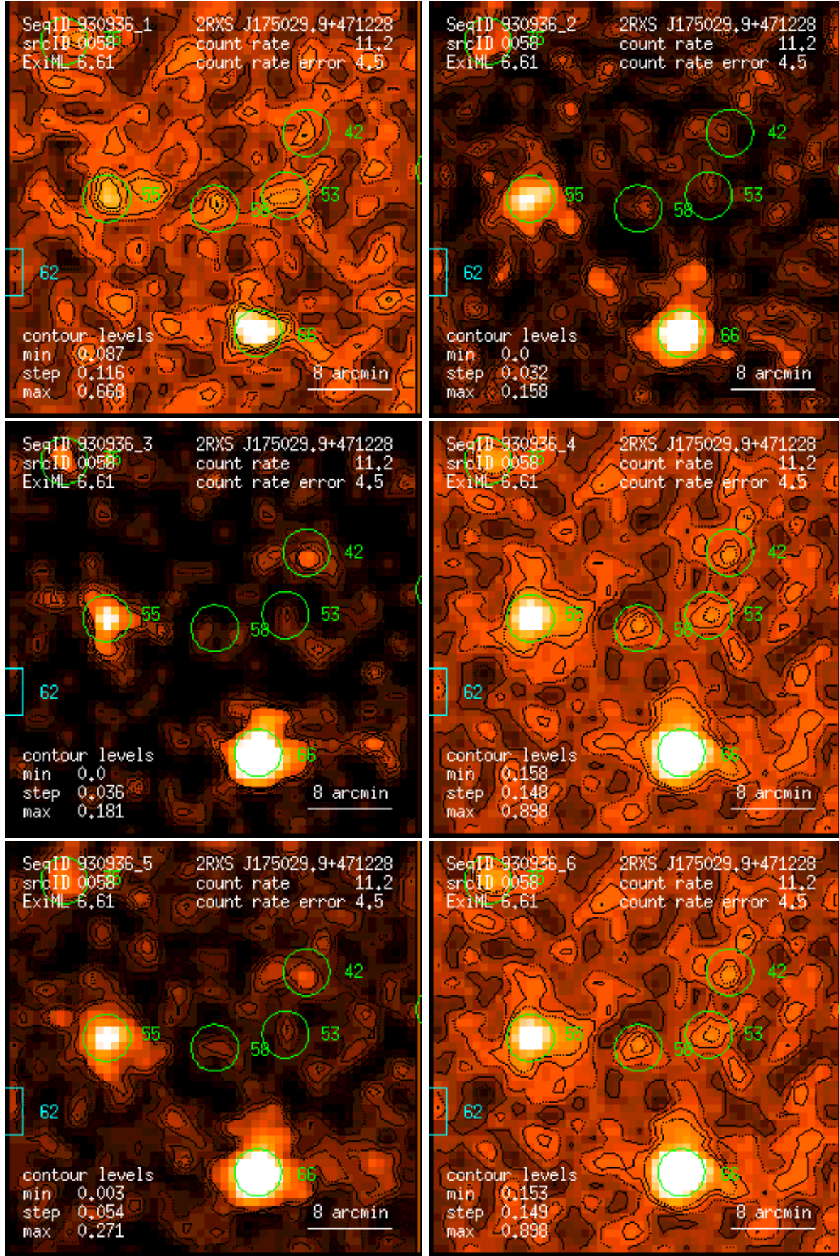
Figure 58: RASS 930936: detection 0058: band rate images, Gaussian filter: (1) PSPC channels 11 – 41, (2) 52 – 90, (3) 91 – 201, (4) 11 – 235, (5) 52 – 201, (6) 11 – 201. Broad band rates in counts/ks. Band rate contour levels in counts/ks/arcmin 2 .
