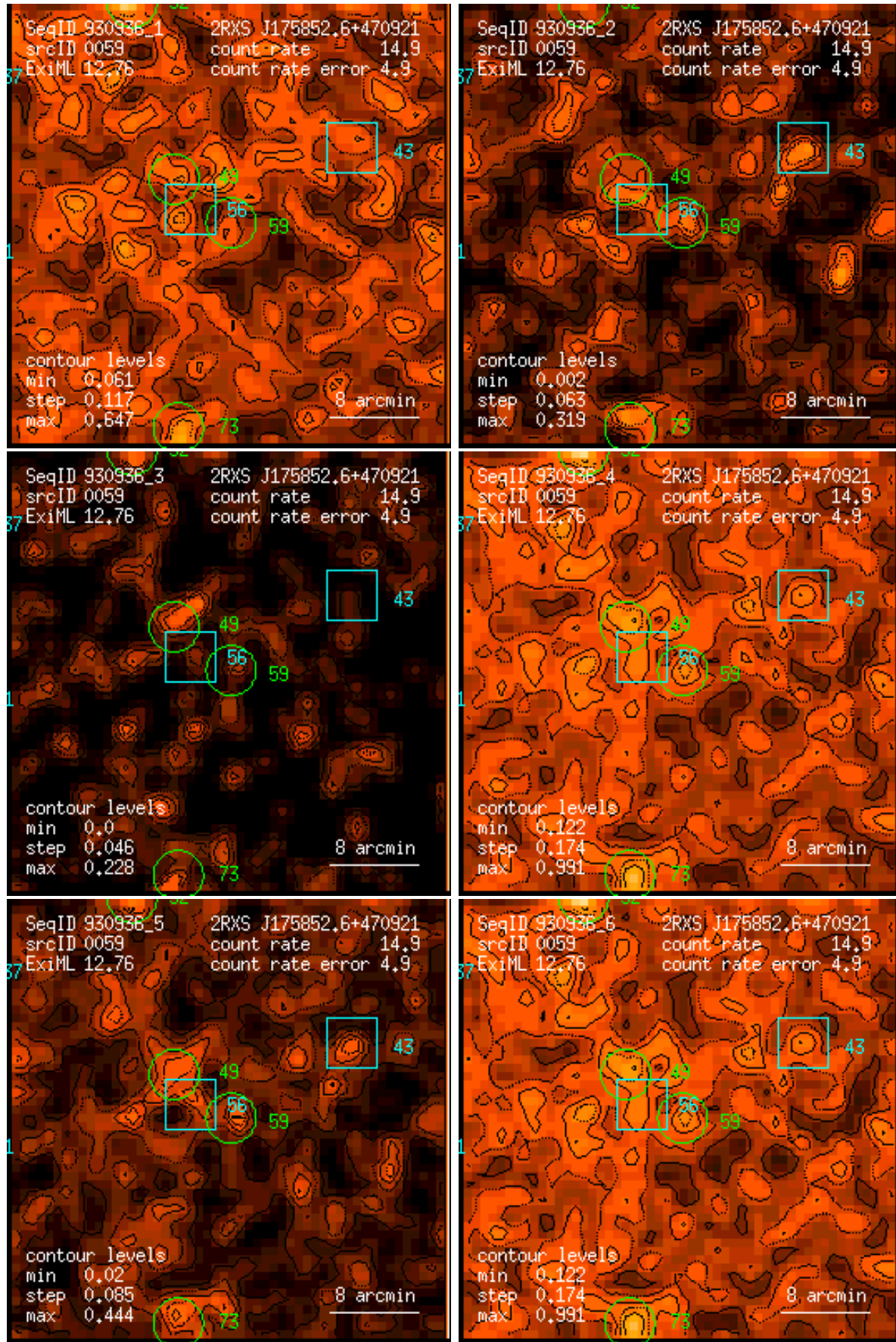
Figure 59: RASS 930936: detection 0059: band rate images, Gaussian filter: (1) PSPC channels 11 – 41, (2) 52 – 90, (3) 91 – 201, (4) 11 – 235, (5) 52 – 201, (6) 11 – 201. Broad band rates in counts/ks. Band rate contour levels in counts/ks/arcmin 2 .
