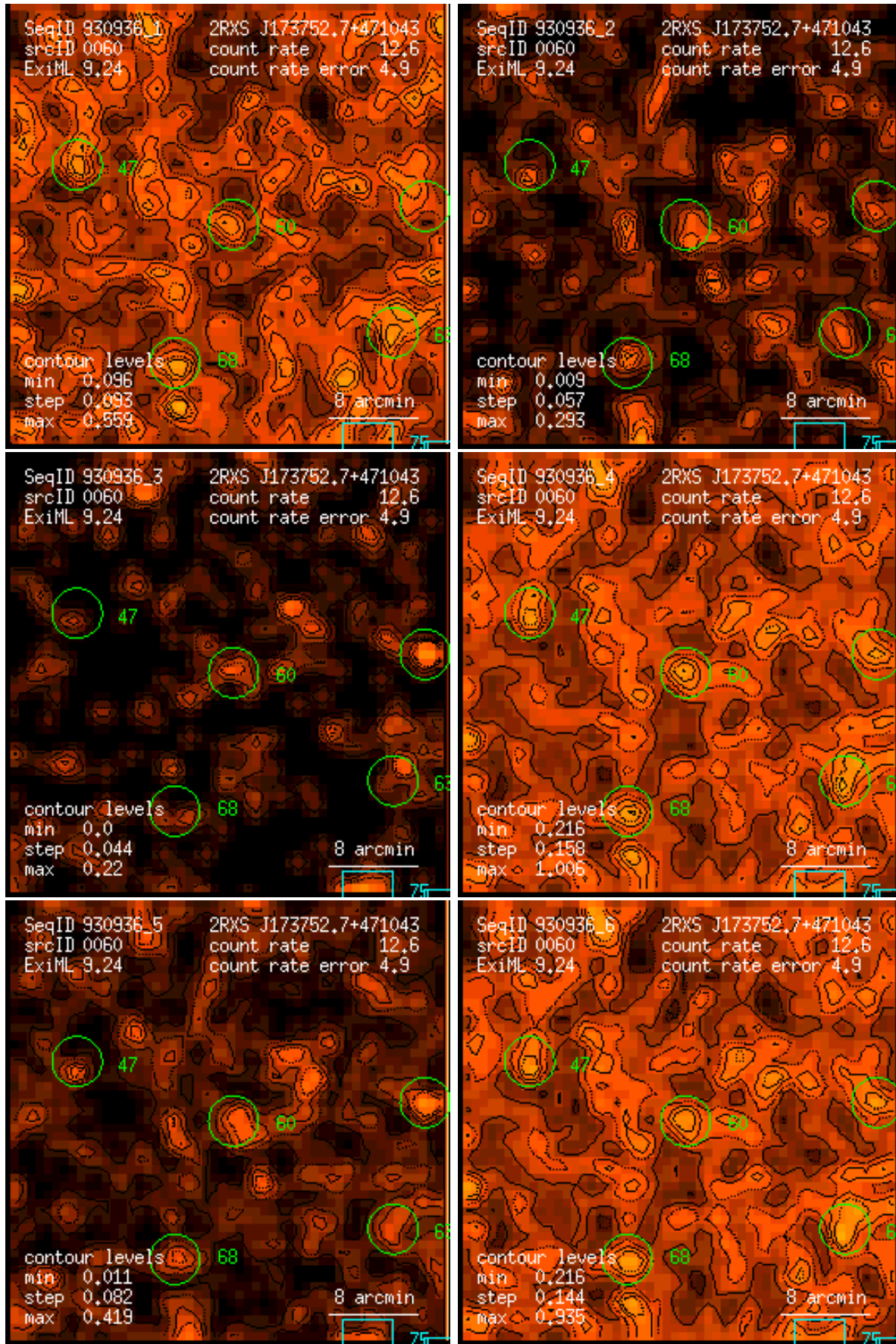
Figure 60: RASS 930936: detection 0060: band rate images, Gaussian filter: (1) PSPC channels 11 – 41, (2) 52 – 90, (3) 91 – 201, (4) 11 – 235, (5) 52 – 201, (6) 11 – 201. Broad band rates in counts/ks. Band rate contour levels in counts/ks/arcmin 2 .
