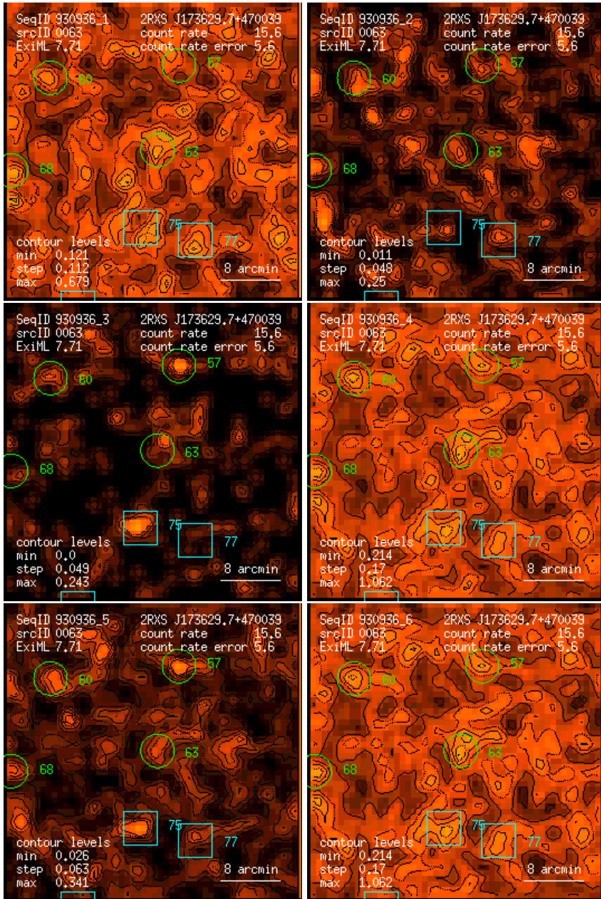
Figure 63: RASS 930936: detection 0063: band rate images, Gaussian filter: (1) PSPC channels 11 – 41, (2) 52 – 90, (3) 91 – 201, (4) 11 – 235, (5) 52 – 201, (6) 11 – 201. Broad band rates in counts/ks. Band rate contour levels in counts/ks/arcmin 2 .
