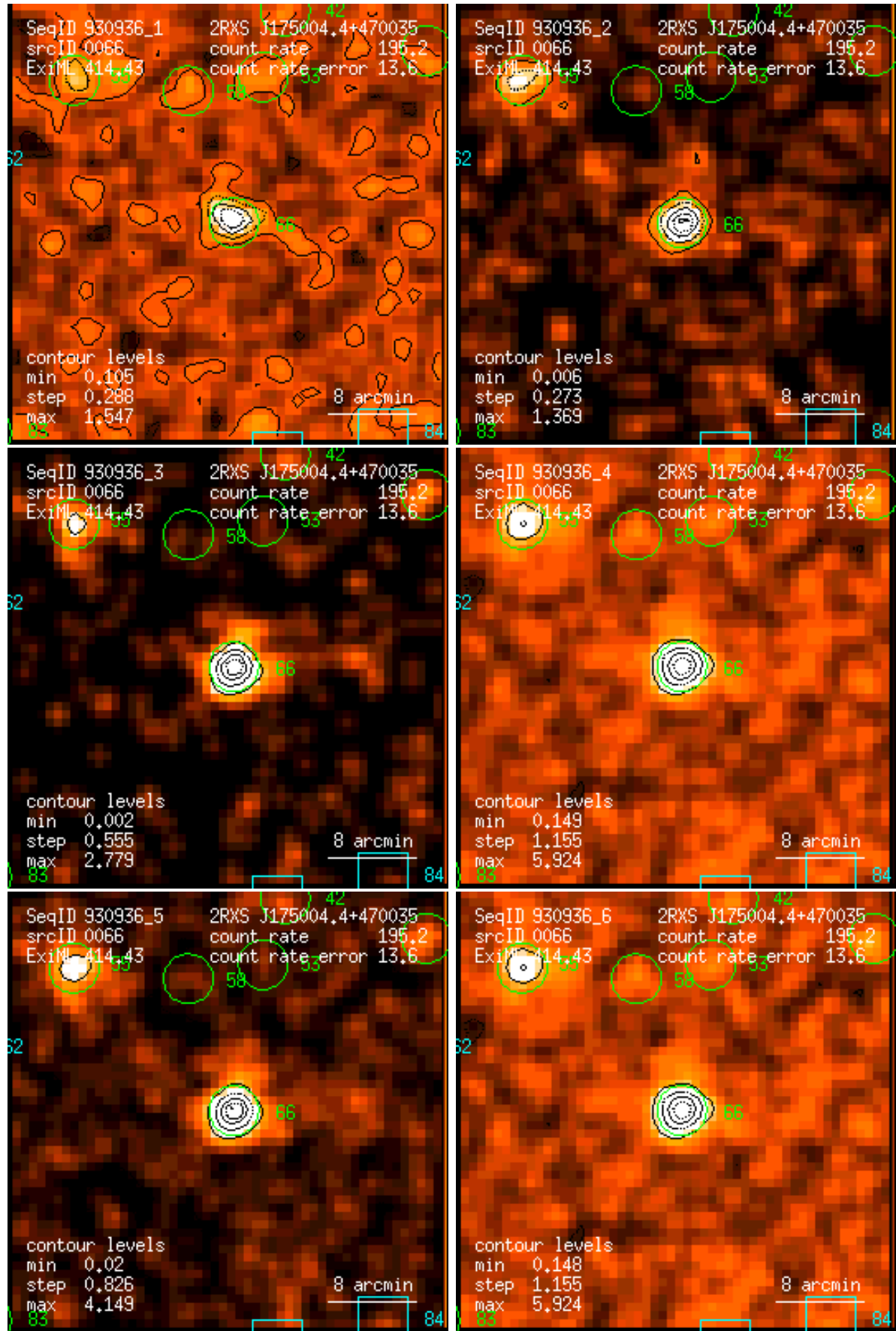
Figure 66: RASS 930936: detection 0066: band rate images, Gaussian filter: (1) PSPC channels 11 – 41, (2) 52 – 90, (3) 91 – 201, (4) 11 – 235, (5) 52 – 201, (6) 11 – 201. Broad band rates in counts/ks. Band rate contour levels in counts/ks/arcmin 2 .
