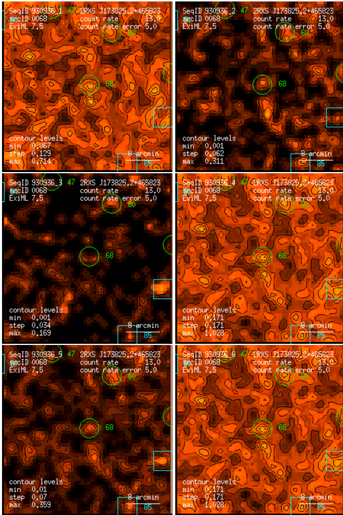
Figure 68: RASS 930936: detection 0068: band rate images, Gaussian filter: (1) PSPC channels 11 – 41, (2) 52 – 90, (3) 91 – 201, (4) 11 – 235, (5) 52 – 201, (6) 11 – 201. Broad band rates in counts/ks. Band rate contour levels in counts/ks/arcmin 2 .
