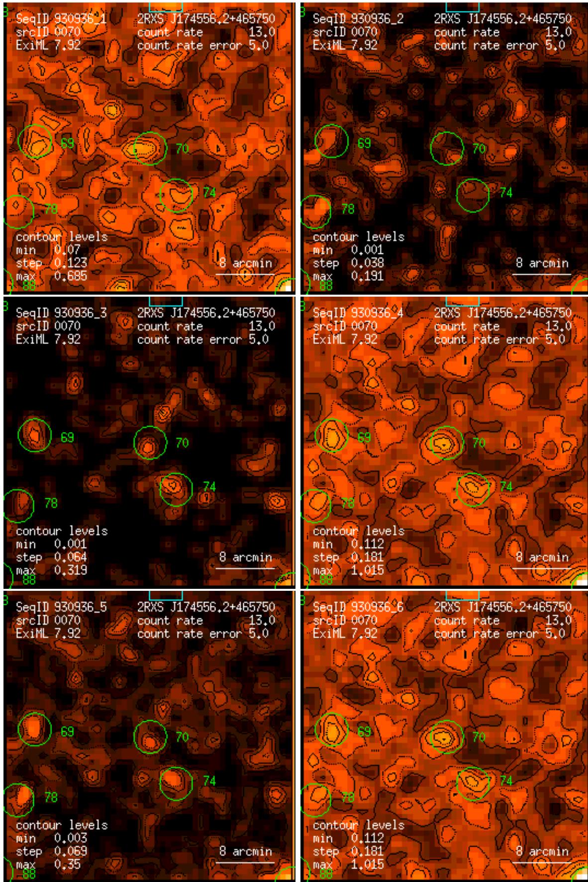
Figure 70: RASS 930936: detection 0070: band rate images, Gaussian filter: (1) PSPC channels 11 – 41, (2) 52 – 90, (3) 91 – 201, (4) 11 – 235, (5) 52 – 201, (6) 11 – 201. Broad band rates in counts/ks. Band rate contour levels in counts/ks/arcmin 2 .
