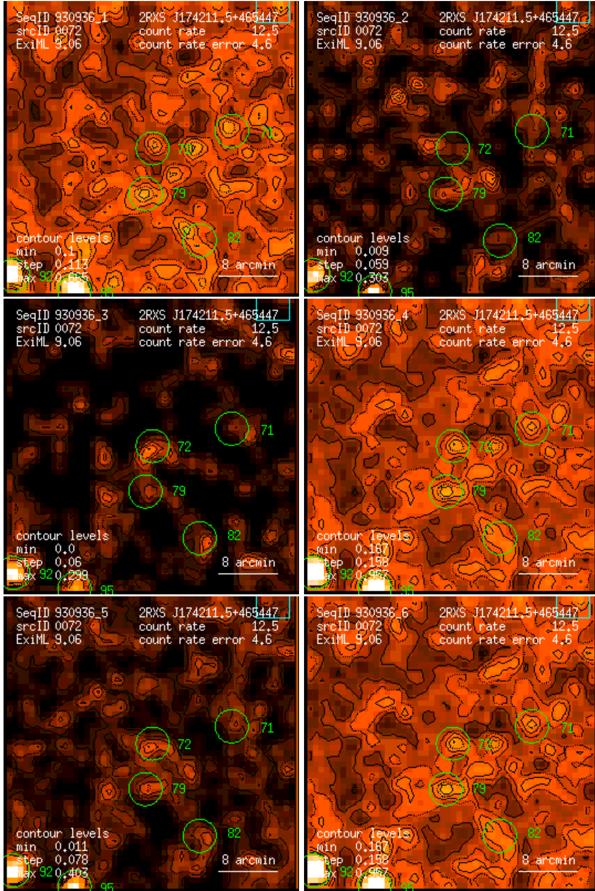
Figure 72: RASS 930936: detection 0072: band rate images, Gaussian filter: (1) PSPC channels 11 – 41, (2) 52 – 90, (3) 91 – 201, (4) 11 – 235, (5) 52 – 201, (6) 11 – 201. Broad band rates in counts/ks. Band rate contour levels in counts/ks/arcmin 2 .
