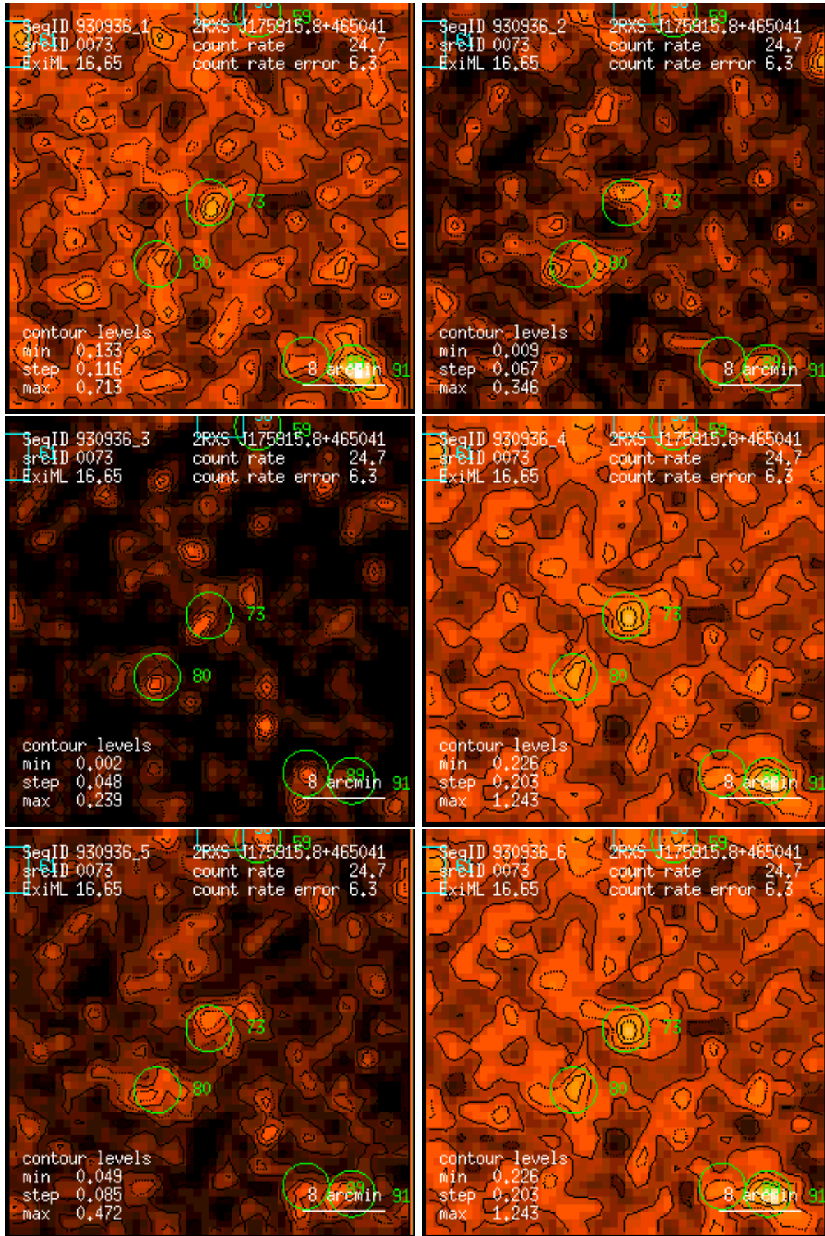
Figure 73: RASS 930936: detection 0073: band rate images, Gaussian filter: (1) PSPC channels 11 – 41, (2) 52 – 90, (3) 91 – 201, (4) 11 – 235, (5) 52 – 201, (6) 11 – 201. Broad band rates in counts/ks. Band rate contour levels in counts/ks/arcmin 2 .
