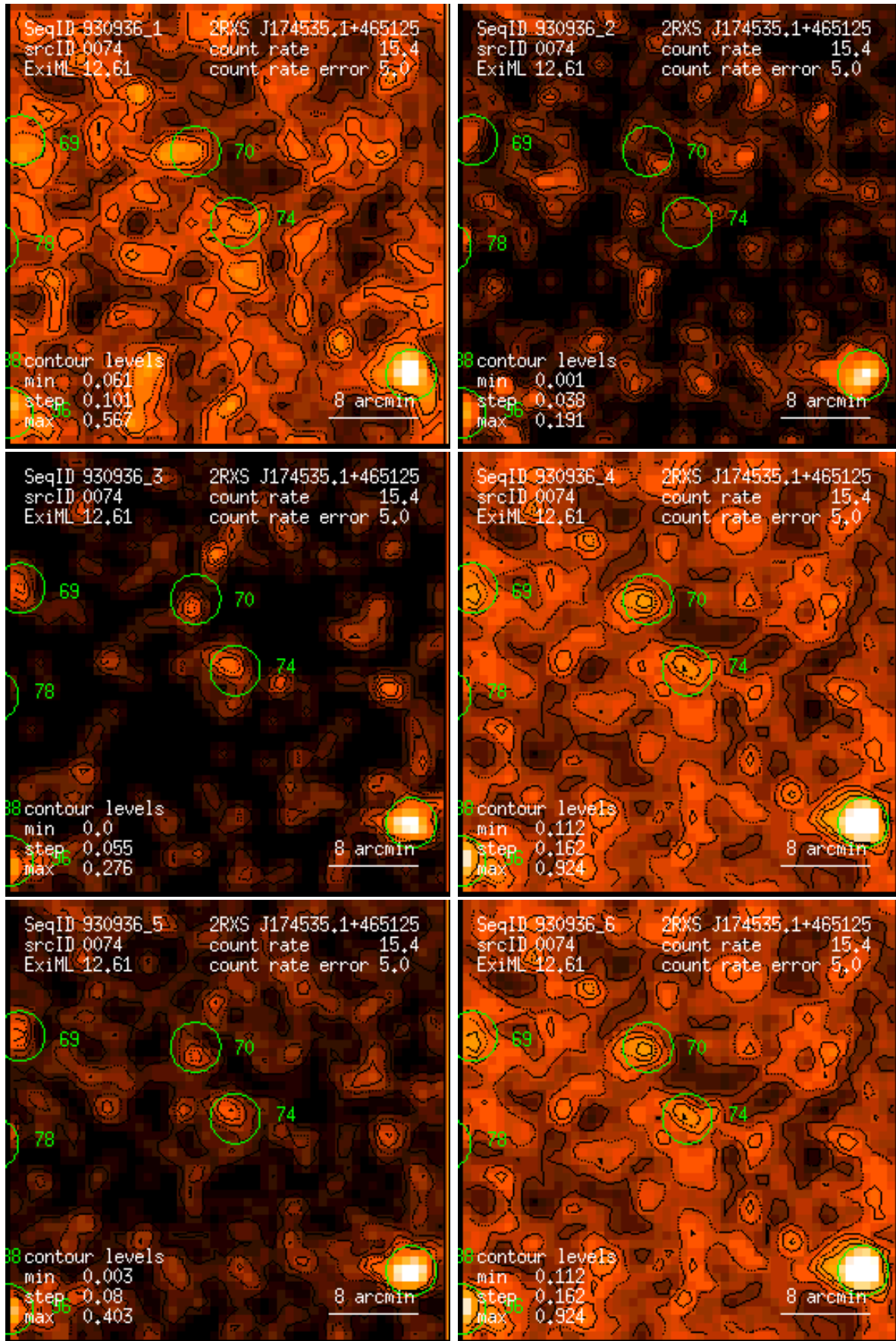
Figure 74: RASS 930936: detection 0074: band rate images, Gaussian filter: (1) PSPC channels 11 – 41, (2) 52 – 90, (3) 91 – 201, (4) 11 – 235, (5) 52 – 201, (6) 11 – 201. Broad band rates in counts/ks. Band rate contour levels in counts/ks/arcmin 2 .
