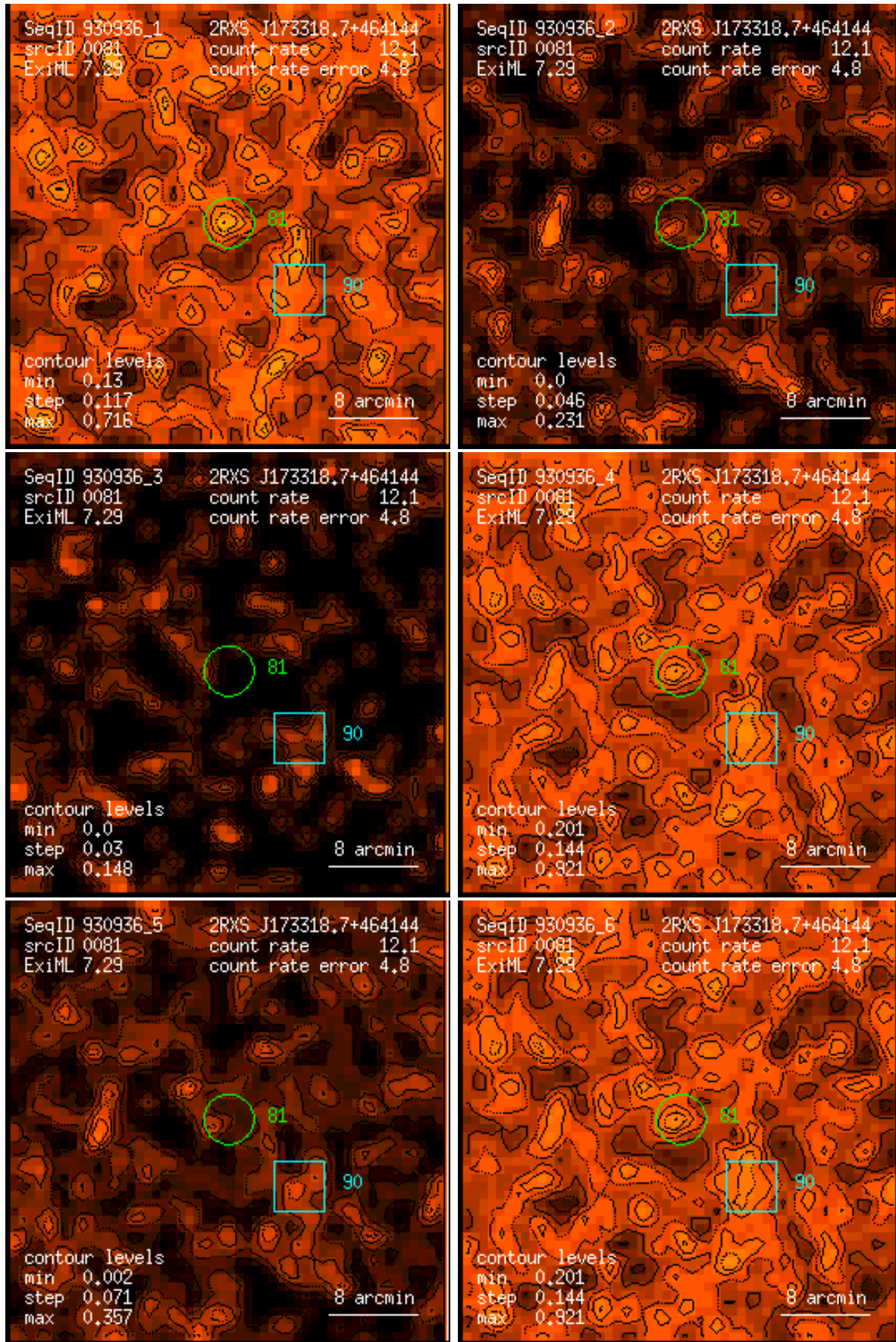
Figure 81: RASS 930936: detection 0081: band rate images, Gaussian filter: (1) PSPC channels 11 – 41, (2) 52 – 90, (3) 91 – 201, (4) 11 – 235, (5) 52 – 201, (6) 11 – 201. Broad band rates in counts/ks. Band rate contour levels in counts/ks/arcmin 2 .
