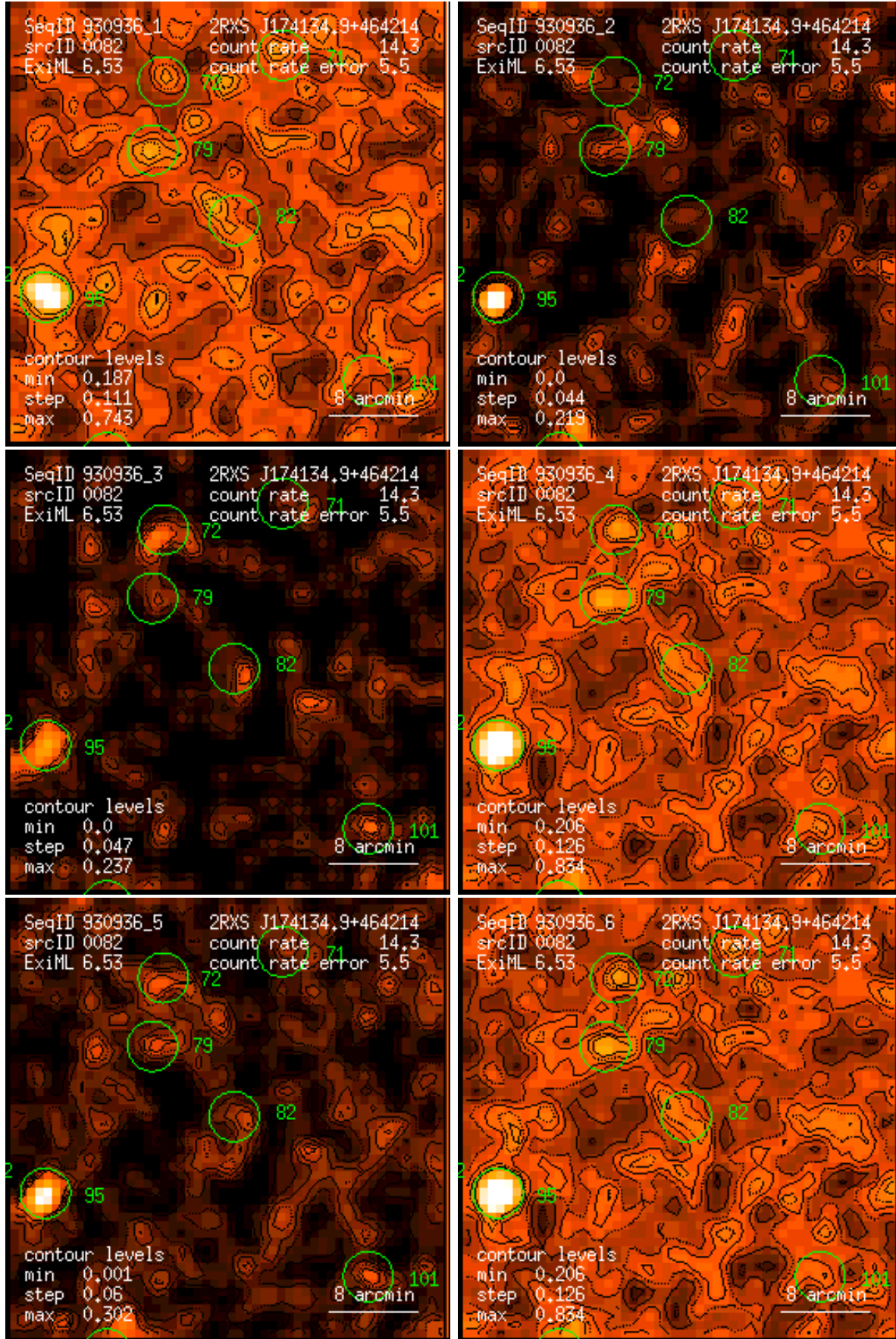
Figure 82: RASS 930936: detection 0082: band rate images, Gaussian filter: (1) PSPC channels 11 – 41, (2) 52 – 90, (3) 91 – 201, (4) 11 – 235, (5) 52 – 201, (6) 11 – 201. Broad band rates in counts/ks. Band rate contour levels in counts/ks/arcmin 2 .
