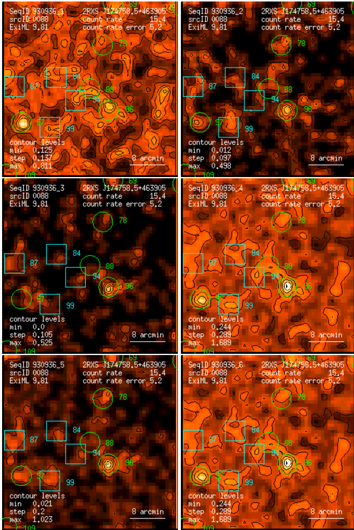
Figure 88: RASS 930936: detection 0088: band rate images, Gaussian filter: (1) PSPC channels 11 – 41, (2) 52 – 90, (3) 91 – 201, (4) 11 – 235, (5) 52 – 201, (6) 11 – 201. Broad band rates in counts/ks. Band rate contour levels in counts/ks/arcmin 2 .
