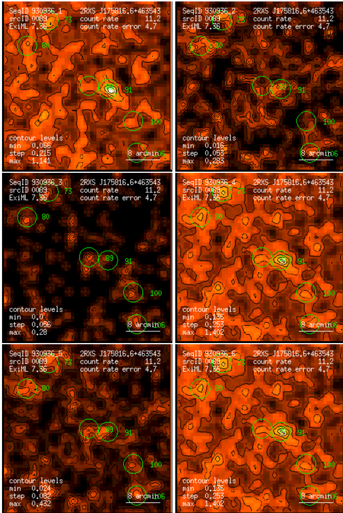
Figure 89: RASS 930936: detection 0089: band rate images, Gaussian filter: (1) PSPC channels 11 – 41, (2) 52 – 90, (3) 91 – 201, (4) 11 – 235, (5) 52 – 201, (6) 11 – 201. Broad band rates in counts/ks. Band rate contour levels in counts/ks/arcmin 2 .
