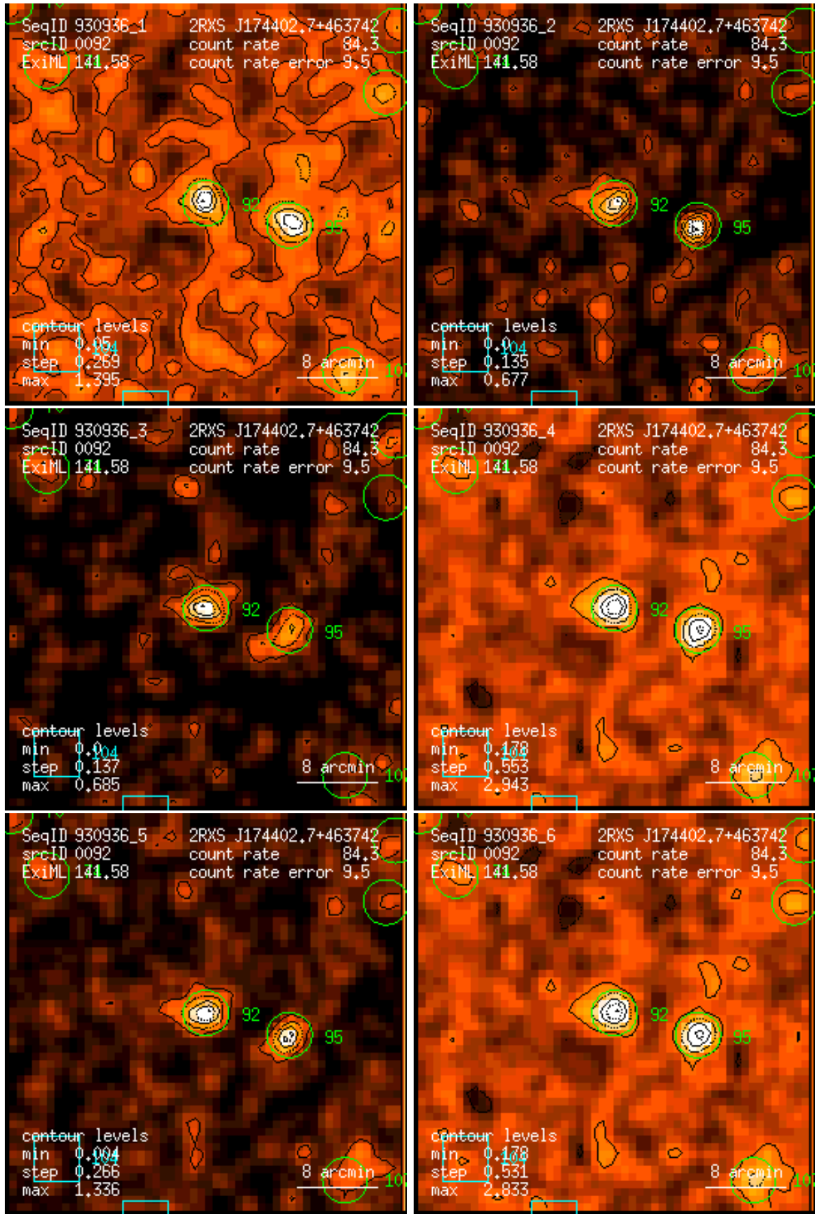
Figure 92: RASS 930936: detection 0092: band rate images, Gaussian filter: (1) PSPC channels 11 – 41, (2) 52 – 90, (3) 91 – 201, (4) 11 – 235, (5) 52 – 201, (6) 11 – 201. Broad band rates in counts/ks. Band rate contour levels in counts/ks/arcmin 2 .
