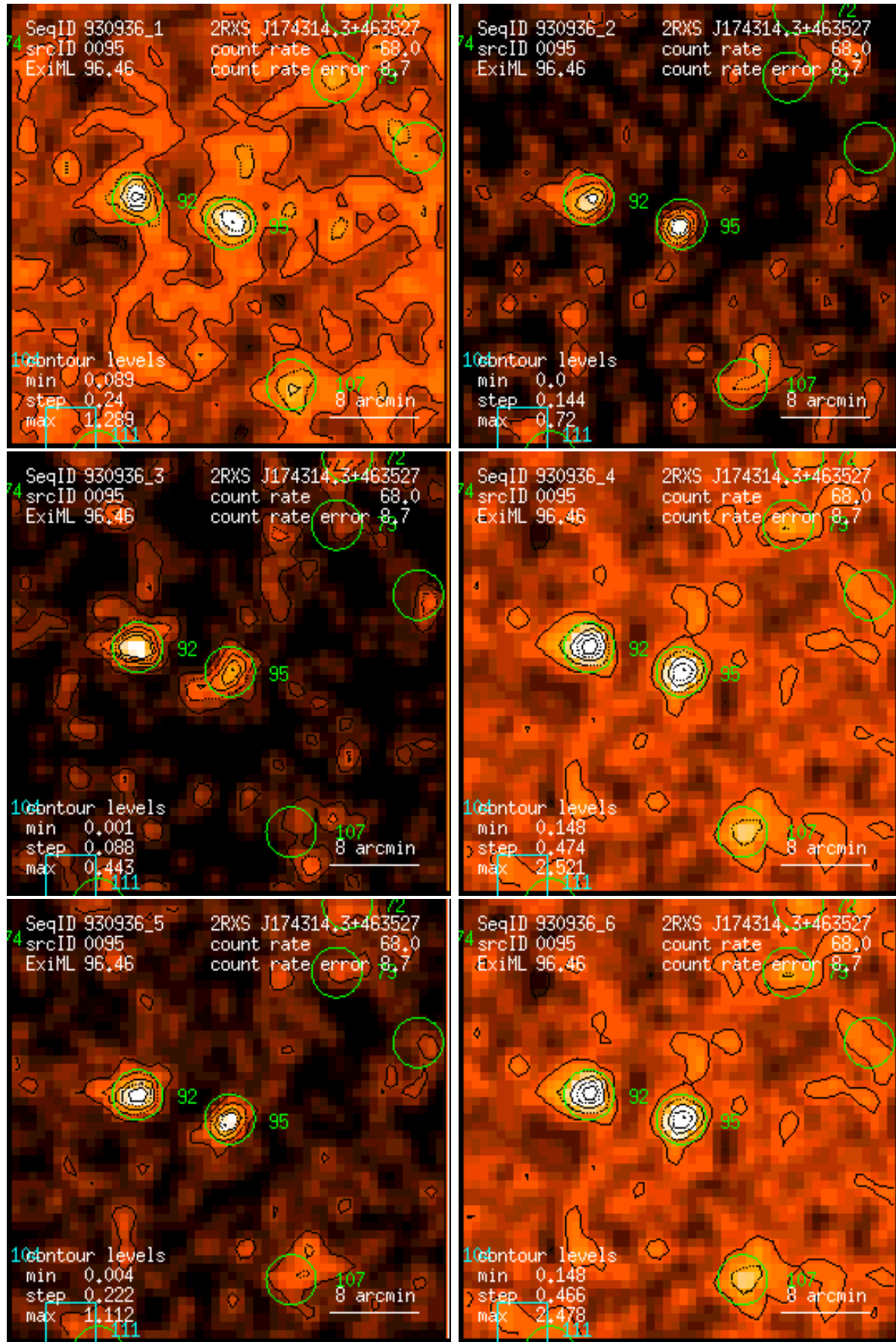
Figure 95: RASS 930936: detection 0095: band rate images, Gaussian filter: (1) PSPC channels 11 – 41, (2) 52 – 90, (3) 91 – 201, (4) 11 – 235, (5) 52 – 201, (6) 11 – 201. Broad band rates in counts/ks. Band rate contour levels in counts/ks/arcmin 2 .
