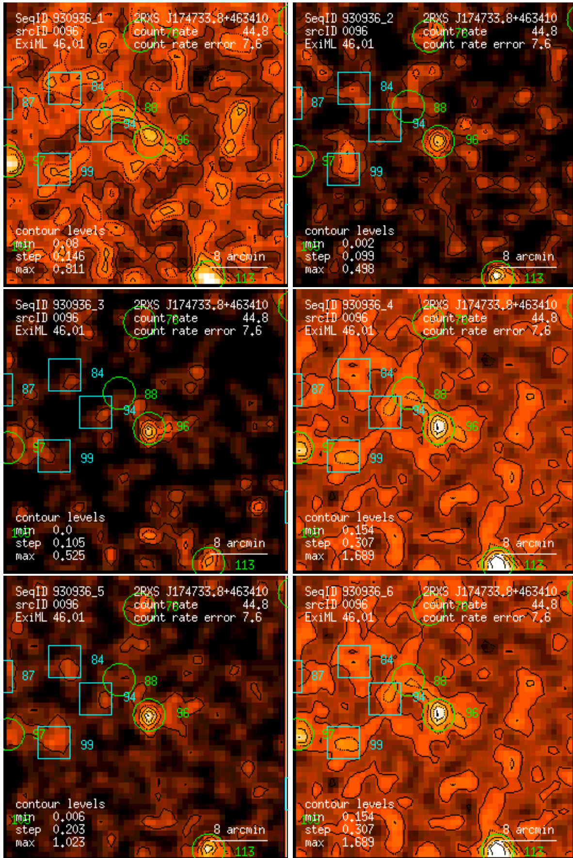
Figure 96: RASS 930936: detection 0096: band rate images, Gaussian filter: (1) PSPC channels 11 – 41, (2) 52 – 90, (3) 91 – 201, (4) 11 – 235, (5) 52 – 201, (6) 11 – 201. Broad band rates in counts/ks. Band rate contour levels in counts/ks/arcmin 2 .
