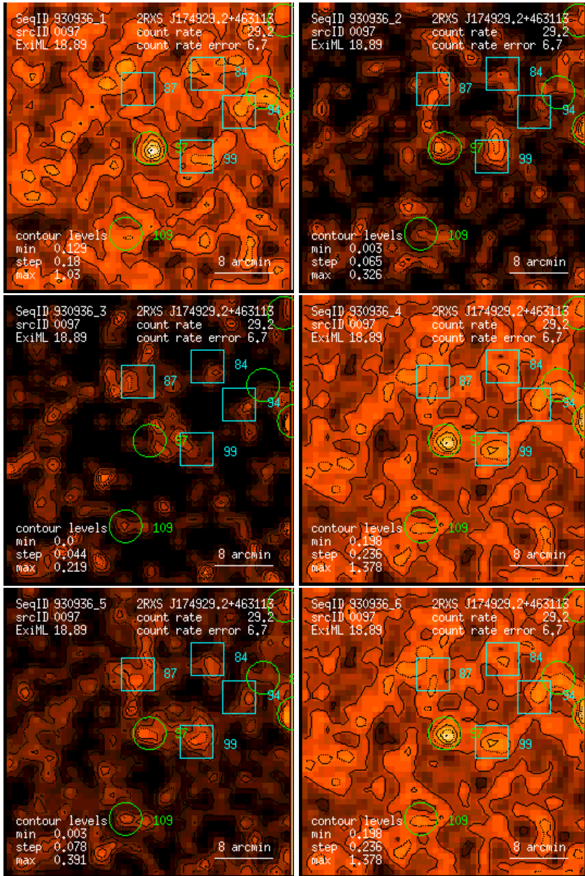
Figure 97: RASS 930936: detection 0097: band rate images, Gaussian filter: (1) PSPC channels 11 – 41, (2) 52 – 90, (3) 91 – 201, (4) 11 – 235, (5) 52 – 201, (6) 11 – 201. Broad band rates in counts/ks. Band rate contour levels in counts/ks/arcmin 2 .
