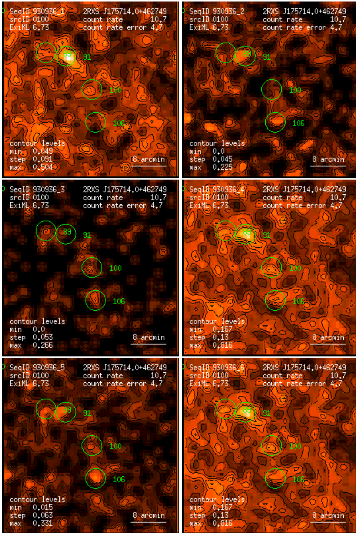
Figure 100: RASS 930936: detection 0100: band rate images, Gaussian filter: (1) PSPC channels 11 – 41, (2) 52 – 90, (3) 91 – 201, (4) 11 – 235, (5) 52 – 201, (6) 11 – 201. Broad band rates in counts/ks. Band rate contour levels in counts/ks/arcmin 2 .
