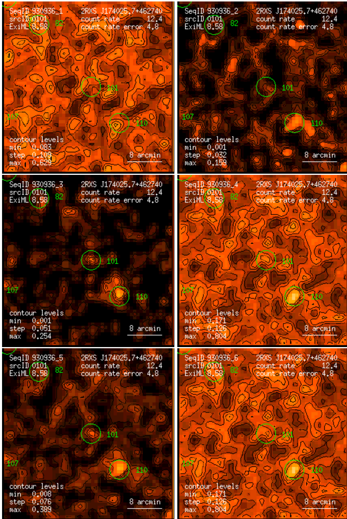
Figure 101: RASS 930936: detection 0101: band rate images, Gaussian filter: (1) PSPC channels 11 – 41, (2) 52 – 90, (3) 91 – 201, (4) 11 – 235, (5) 52 – 201, (6) 11 – 201. Broad band rates in counts/ks. Band rate contour levels in counts/ks/arcmin 2 .
