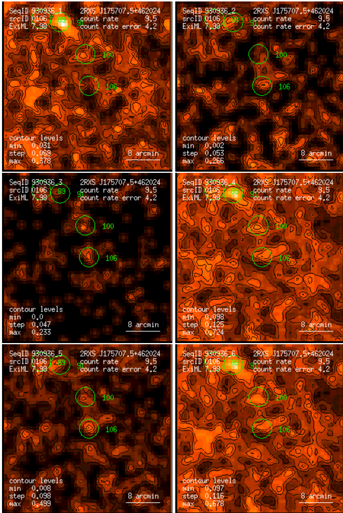
Figure 106: RASS 930936: detection 0106: band rate images, Gaussian filter: (1) PSPC channels 11 – 41, (2) 52 – 90, (3) 91 – 201, (4) 11 – 235, (5) 52 – 201, (6) 11 – 201. Broad band rates in counts/ks. Band rate contour levels in counts/ks/arcmin 2 .
