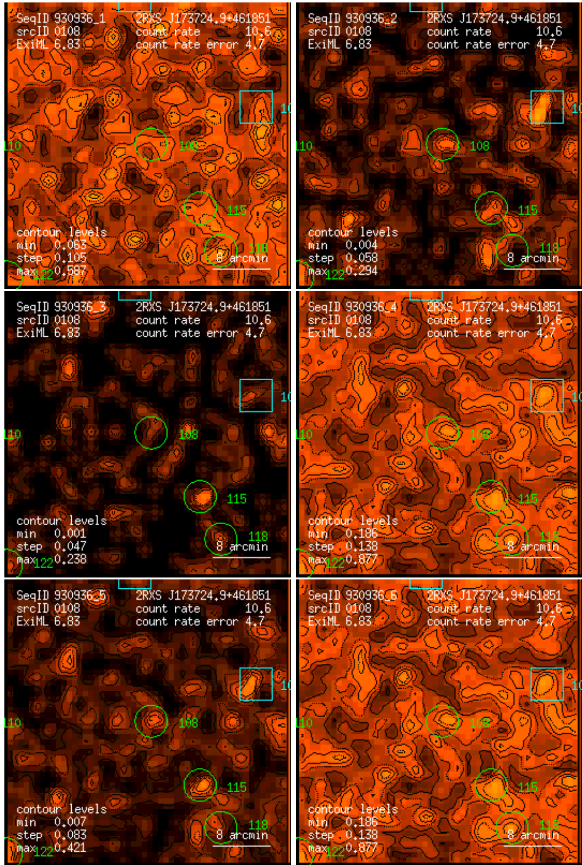
Figure 108: RASS 930936: detection 0108: band rate images, Gaussian filter: (1) PSPC channels 11 – 41, (2) 52 – 90, (3) 91 – 201, (4) 11 – 235, (5) 52 – 201, (6) 11 – 201. Broad band rates in counts/ks. Band rate contour levels in counts/ks/arcmin 2 .
