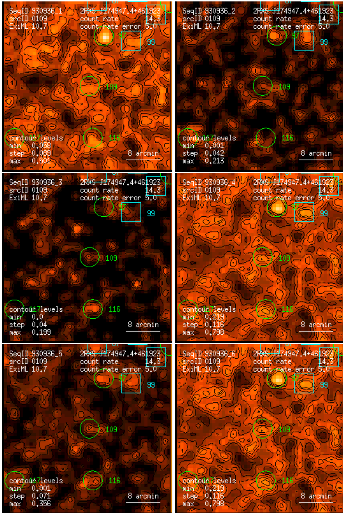
Figure 109: RASS 930936: detection 0109: band rate images, Gaussian filter: (1) PSPC channels 11 – 41, (2) 52 – 90, (3) 91 – 201, (4) 11 – 235, (5) 52 – 201, (6) 11 – 201. Broad band rates in counts/ks. Band rate contour levels in counts/ks/arcmin 2 .
