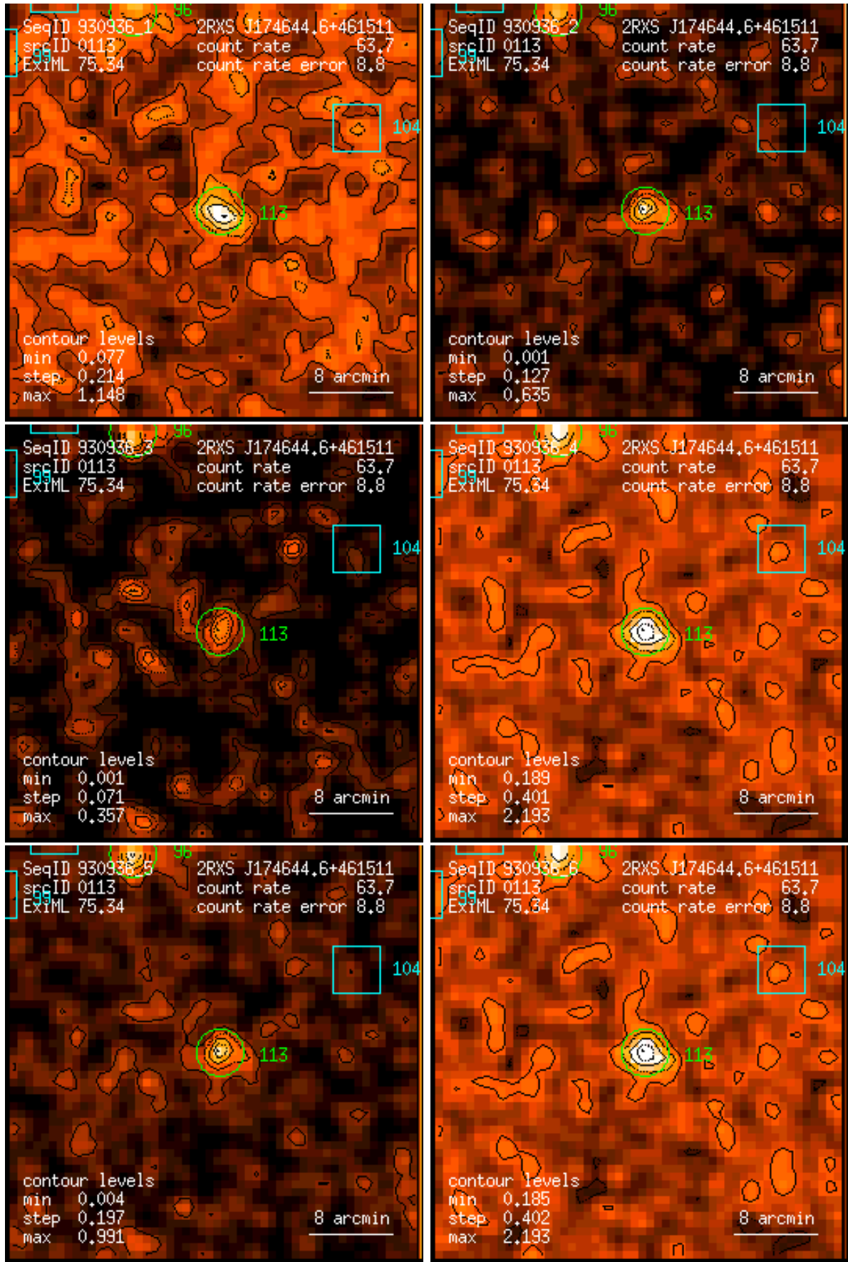
Figure 113: RASS 930936: detection 0113: band rate images, Gaussian filter: (1) PSPC channels 11 – 41, (2) 52 – 90, (3) 91 – 201, (4) 11 – 235, (5) 52 – 201, (6) 11 – 201. Broad band rates in counts/ks. Band rate contour levels in counts/ks/arcmin 2 .
