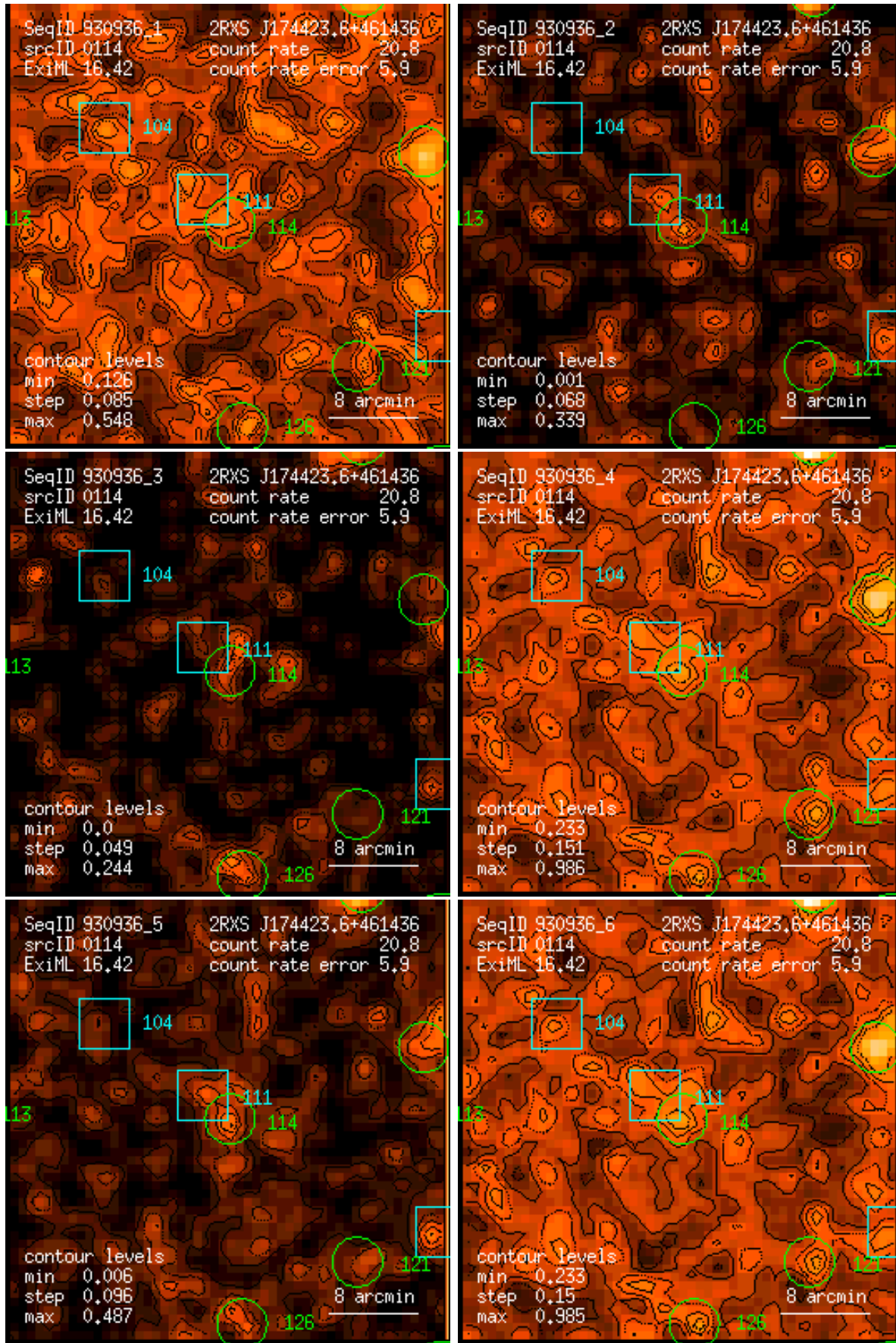
Figure 114: RASS 930936: detection 0114: band rate images, Gaussian filter: (1) PSPC channels 11 – 41, (2) 52 – 90, (3) 91 – 201, (4) 11 – 235, (5) 52 – 201, (6) 11 – 201. Broad band rates in counts/ks. Band rate contour levels in counts/ks/arcmin 2 .
