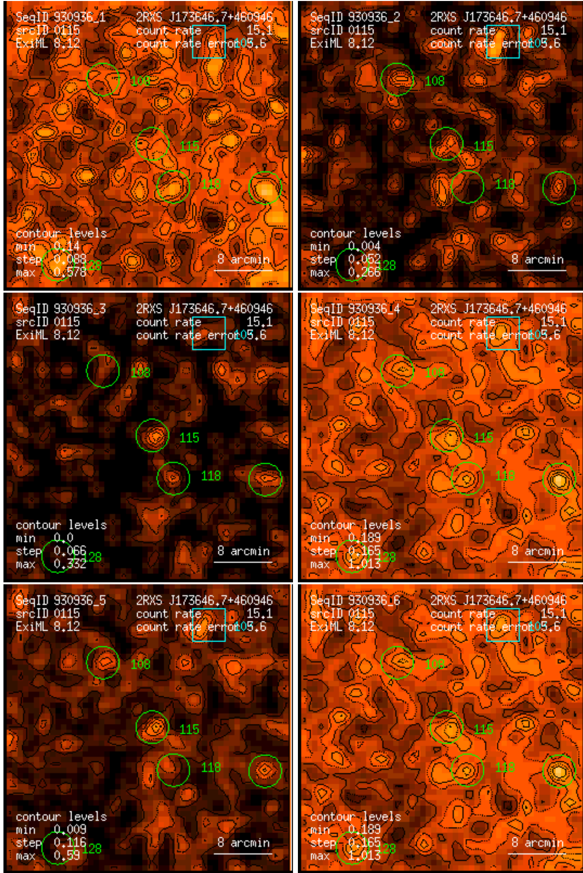
Figure 115: RASS 930936: detection 0115: band rate images, Gaussian filter: (1) PSPC channels 11 – 41, (2) 52 – 90, (3) 91 – 201, (4) 11 – 235, (5) 52 – 201, (6) 11 – 201. Broad band rates in counts/ks. Band rate contour levels in counts/ks/arcmin 2 .
