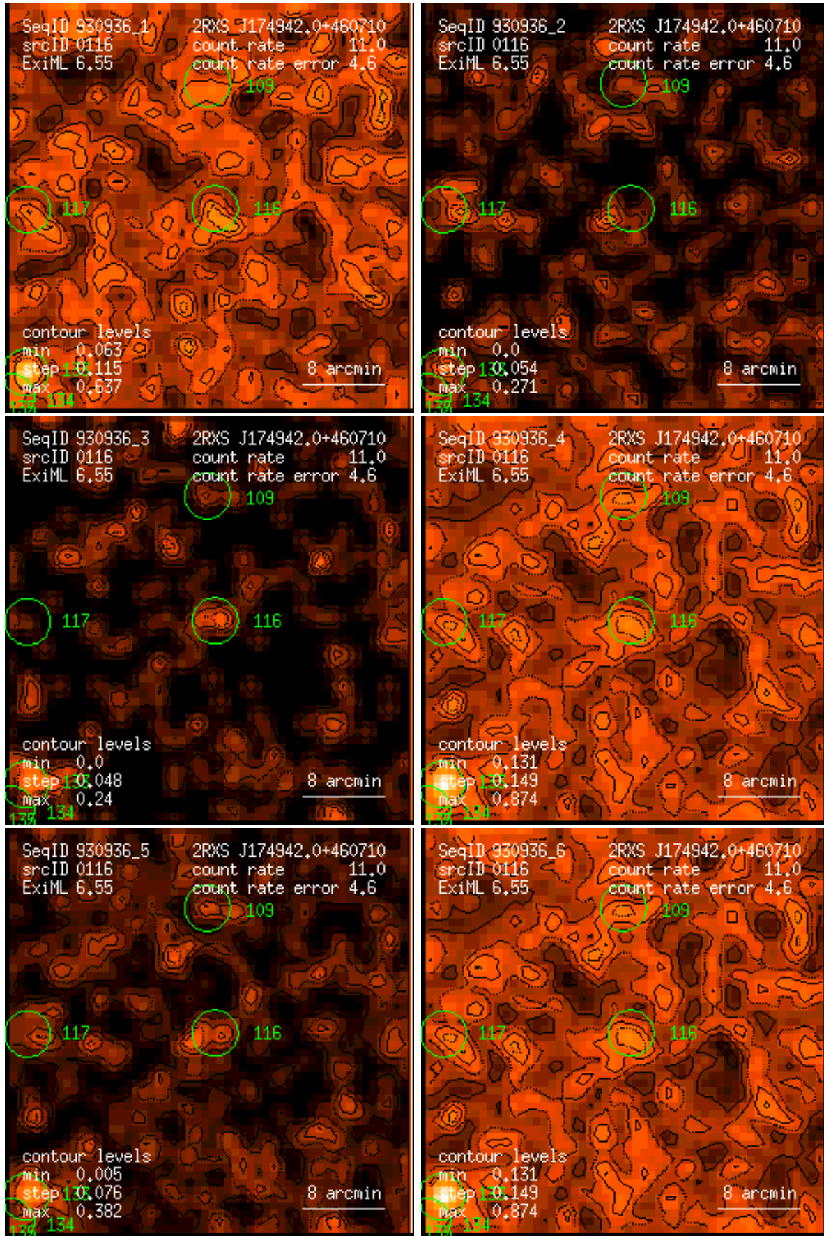
Figure 116: RASS 930936: detection 0116: band rate images, Gaussian filter: (1) PSPC channels 11 – 41, (2) 52 – 90, (3) 91 – 201, (4) 11 – 235, (5) 52 – 201, (6) 11 – 201. Broad band rates in counts/ks. Band rate contour levels in counts/ks/arcmin 2 .
