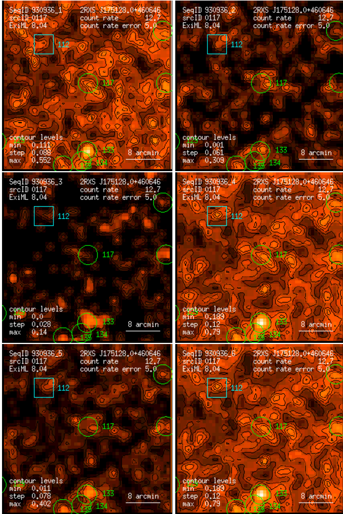
Figure 117: RASS 930936: detection 0117: band rate images, Gaussian filter: (1) PSPC channels 11 – 41, (2) 52 – 90, (3) 91 – 201, (4) 11 – 235, (5) 52 – 201, (6) 11 – 201. Broad band rates in counts/ks. Band rate contour levels in counts/ks/arcmin 2 .
