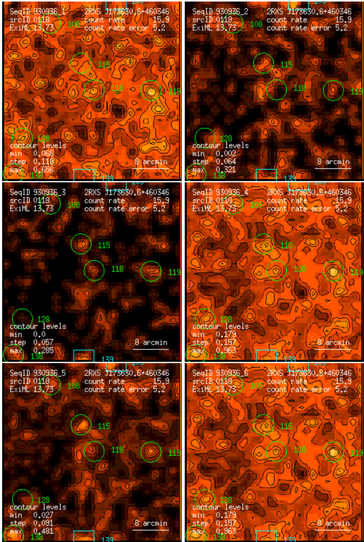
Figure 118: RASS 930936: detection 0118: band rate images, Gaussian filter: (1) PSPC channels 11 – 41, (2) 52 – 90, (3) 91 – 201, (4) 11 – 235, (5) 52 – 201, (6) 11 – 201. Broad band rates in counts/ks. Band rate contour levels in counts/ks/arcmin 2 .
