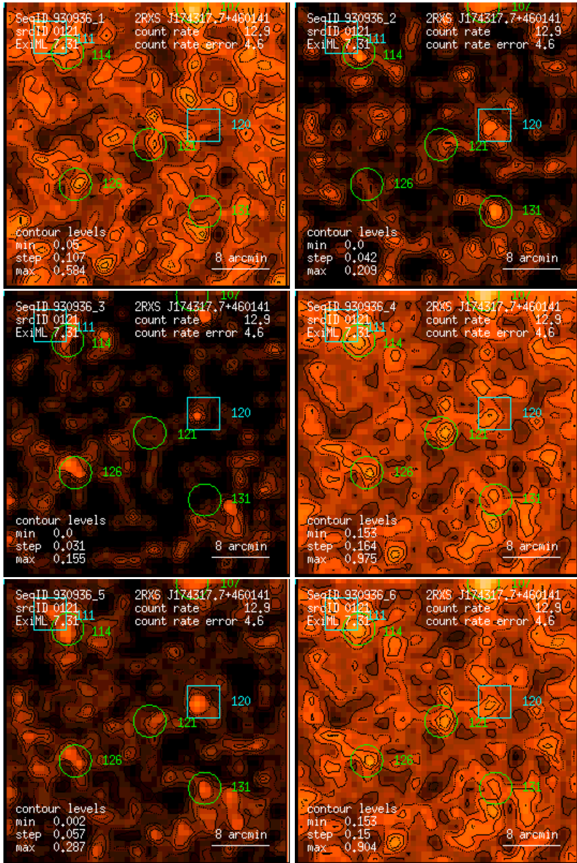
Figure 121: RASS 930936: detection 0121: band rate images, Gaussian filter: (1) PSPC channels 11 – 41, (2) 52 – 90, (3) 91 – 201, (4) 11 – 235, (5) 52 – 201, (6) 11 – 201. Broad band rates in counts/ks. Band rate contour levels in counts/ks/arcmin 2 .
