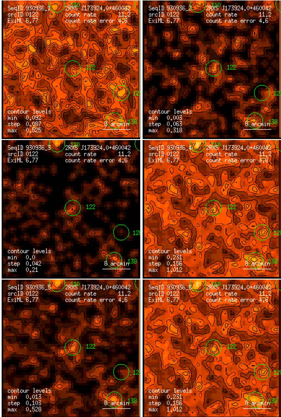
Figure 122: RASS 930936: detection 0122: band rate images, Gaussian filter: (1) PSPC channels 11 – 41, (2) 52 – 90, (3) 91 – 201, (4) 11 – 235, (5) 52 – 201, (6) 11 – 201. Broad band rates in counts/ks. Band rate contour levels in counts/ks/arcmin 2 .
