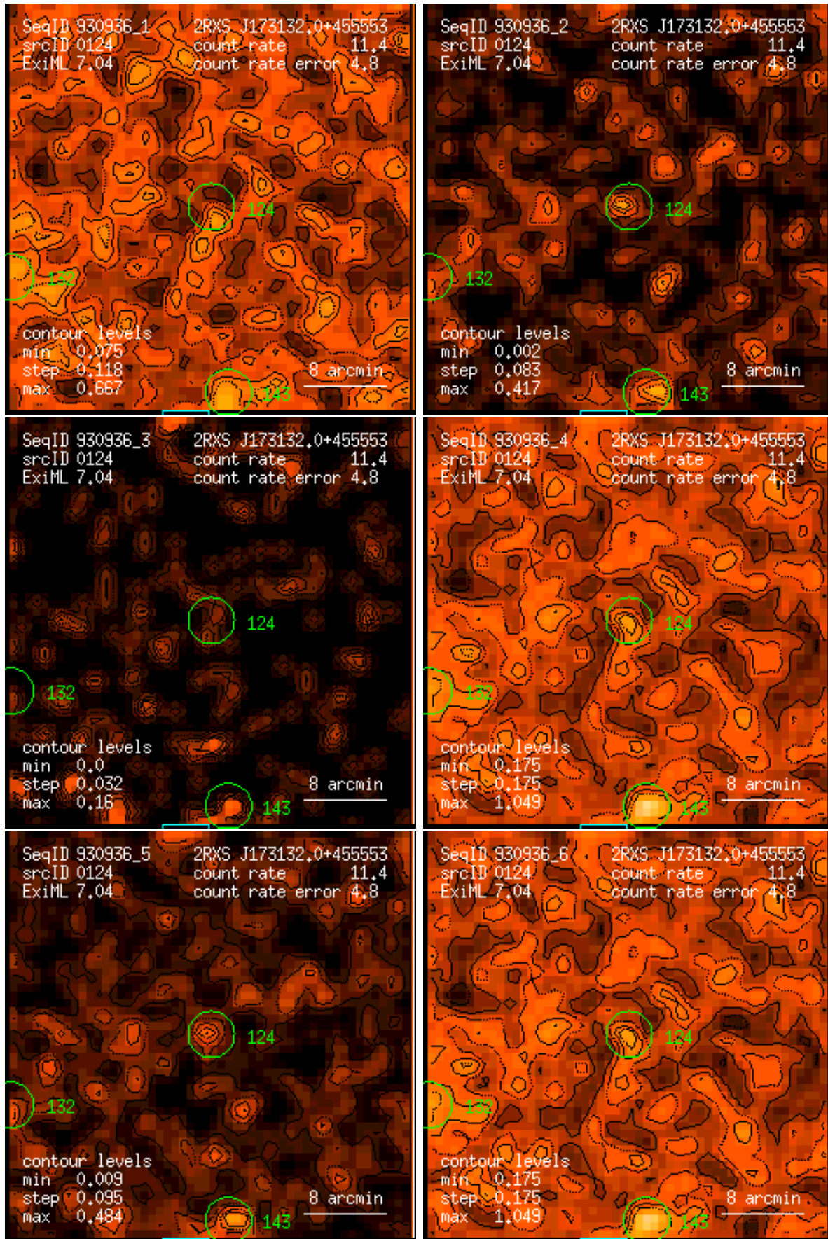
Figure 124: RASS 930936: detection 0124: band rate images, Gaussian filter: (1) PSPC channels 11 – 41, (2) 52 – 90, (3) 91 – 201, (4) 11 – 235, (5) 52 – 201, (6) 11 – 201. Broad band rates in counts/ks. Band rate contour levels in counts/ks/arcmin 2 .
