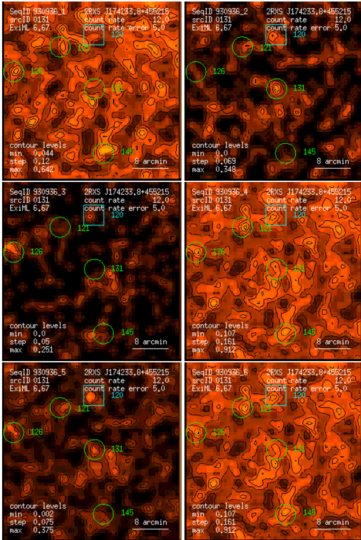
Figure 131: RASS 930936: detection 0131: band rate images, Gaussian filter: (1) PSPC channels 11 – 41, (2) 52 – 90, (3) 91 – 201, (4) 11 – 235, (5) 52 – 201, (6) 11 – 201. Broad band rates in counts/ks. Band rate contour levels in counts/ks/arcmin 2 .
