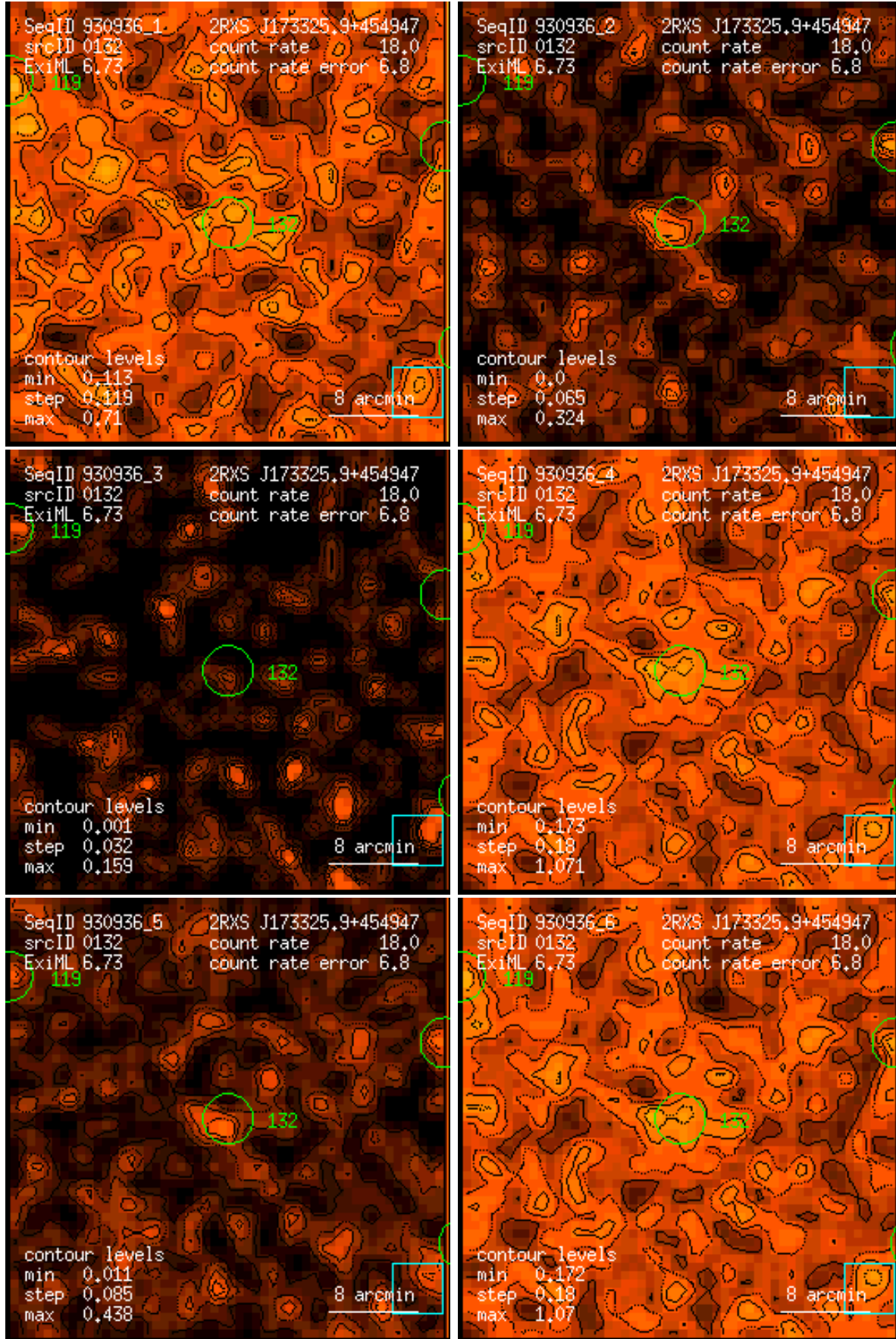
Figure 132: RASS 930936: detection 0132: band rate images, Gaussian filter: (1) PSPC channels 11 – 41, (2) 52 – 90, (3) 91 – 201, (4) 11 – 235, (5) 52 – 201, (6) 11 – 201. Broad band rates in counts/ks. Band rate contour levels in counts/ks/arcmin 2 .
