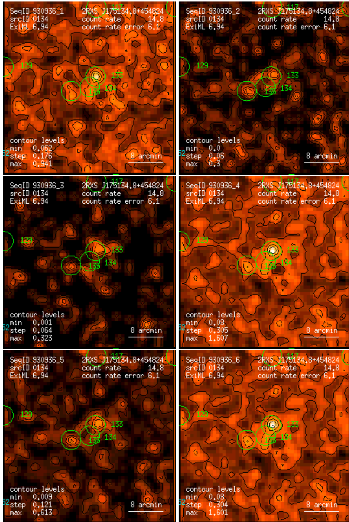
Figure 134: RASS 930936: detection 0134: band rate images, Gaussian filter: (1) PSPC channels 11 – 41, (2) 52 – 90, (3) 91 – 201, (4) 11 – 235, (5) 52 – 201, (6) 11 – 201. Broad band rates in counts/ks. Band rate contour levels in counts/ks/arcmin 2 .
