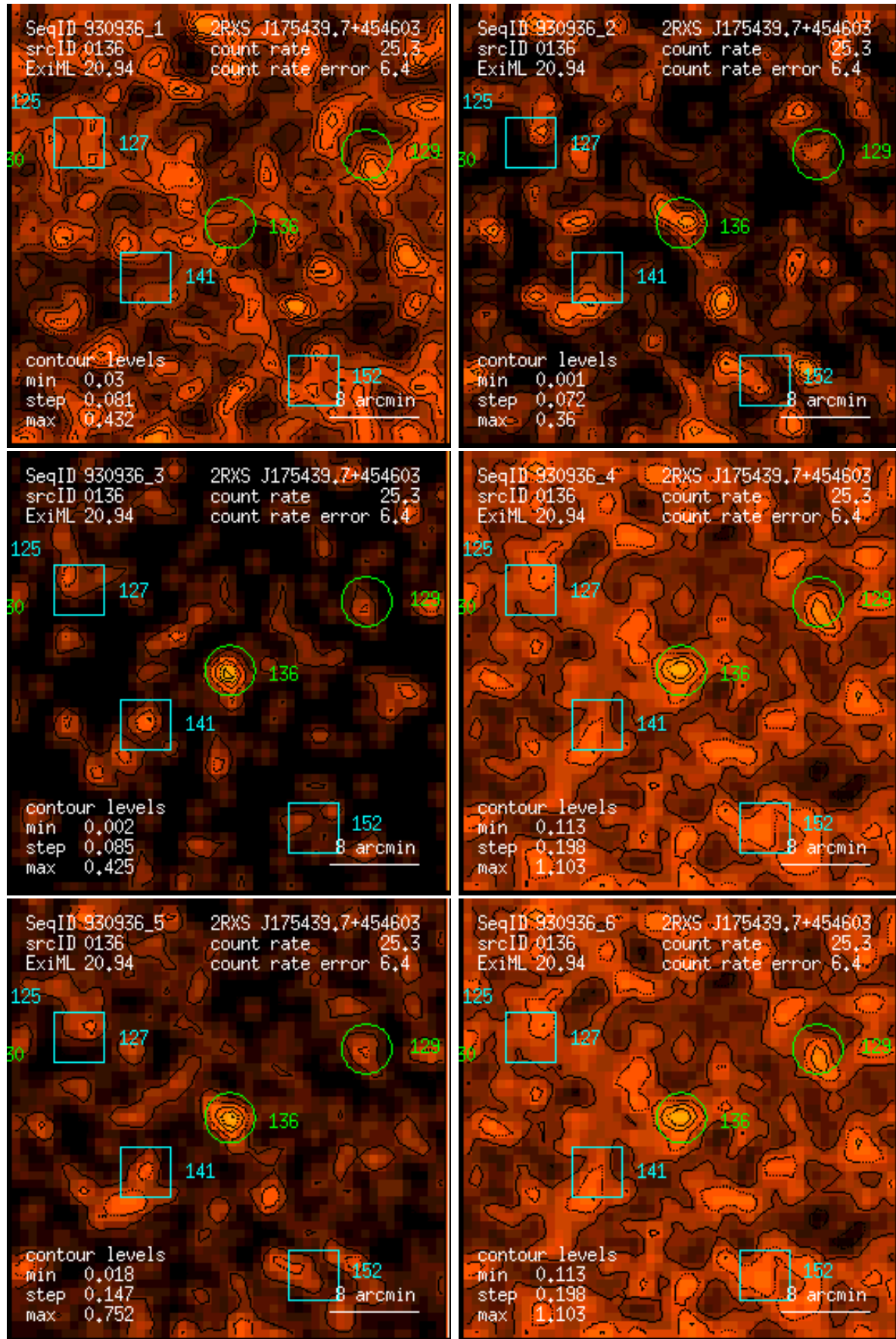
Figure 136: RASS 930936: detection 0136: band rate images, Gaussian filter: (1) PSPC channels 11 – 41, (2) 52 – 90, (3) 91 – 201, (4) 11 – 235, (5) 52 – 201, (6) 11 – 201. Broad band rates in counts/ks. Band rate contour levels in counts/ks/arcmin 2 .
