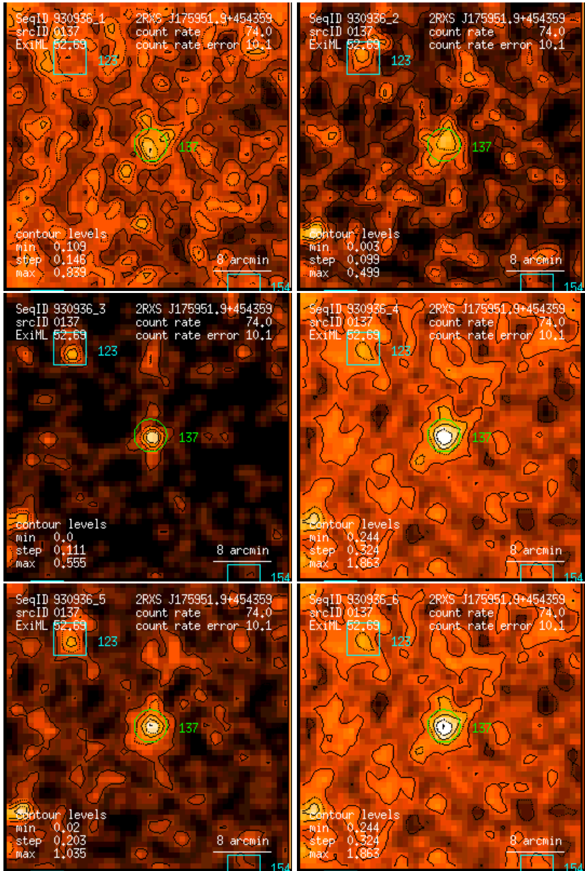
Figure 137: RASS 930936: detection 0137: band rate images, Gaussian filter: (1) PSPC channels 11 – 41, (2) 52 – 90, (3) 91 – 201, (4) 11 – 235, (5) 52 – 201, (6) 11 – 201. Broad band rates in counts/ks. Band rate contour levels in counts/ks/arcmin 2 .
