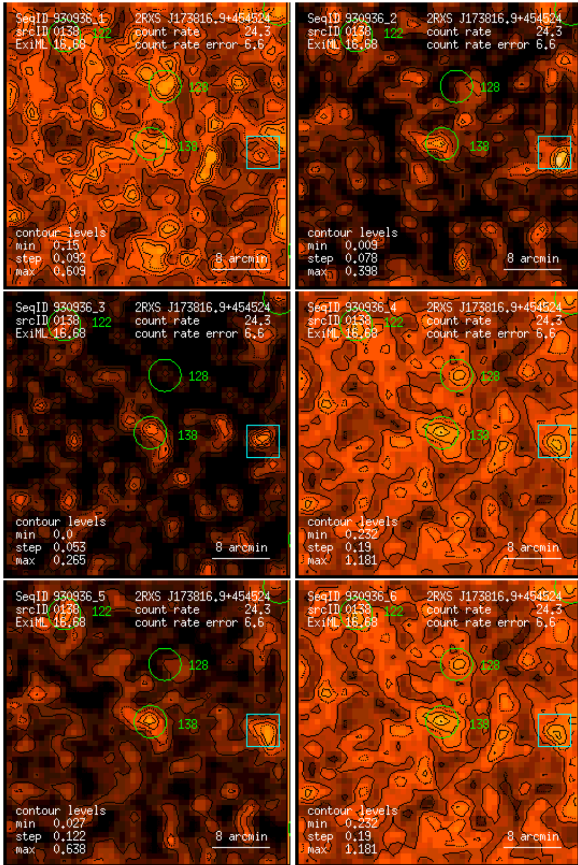
Figure 138: RASS 930936: detection 0138: band rate images, Gaussian filter: (1) PSPC channels 11 – 41, (2) 52 – 90, (3) 91 – 201, (4) 11 – 235, (5) 52 – 201, (6) 11 – 201. Broad band rates in counts/ks. Band rate contour levels in counts/ks/arcmin 2 .
