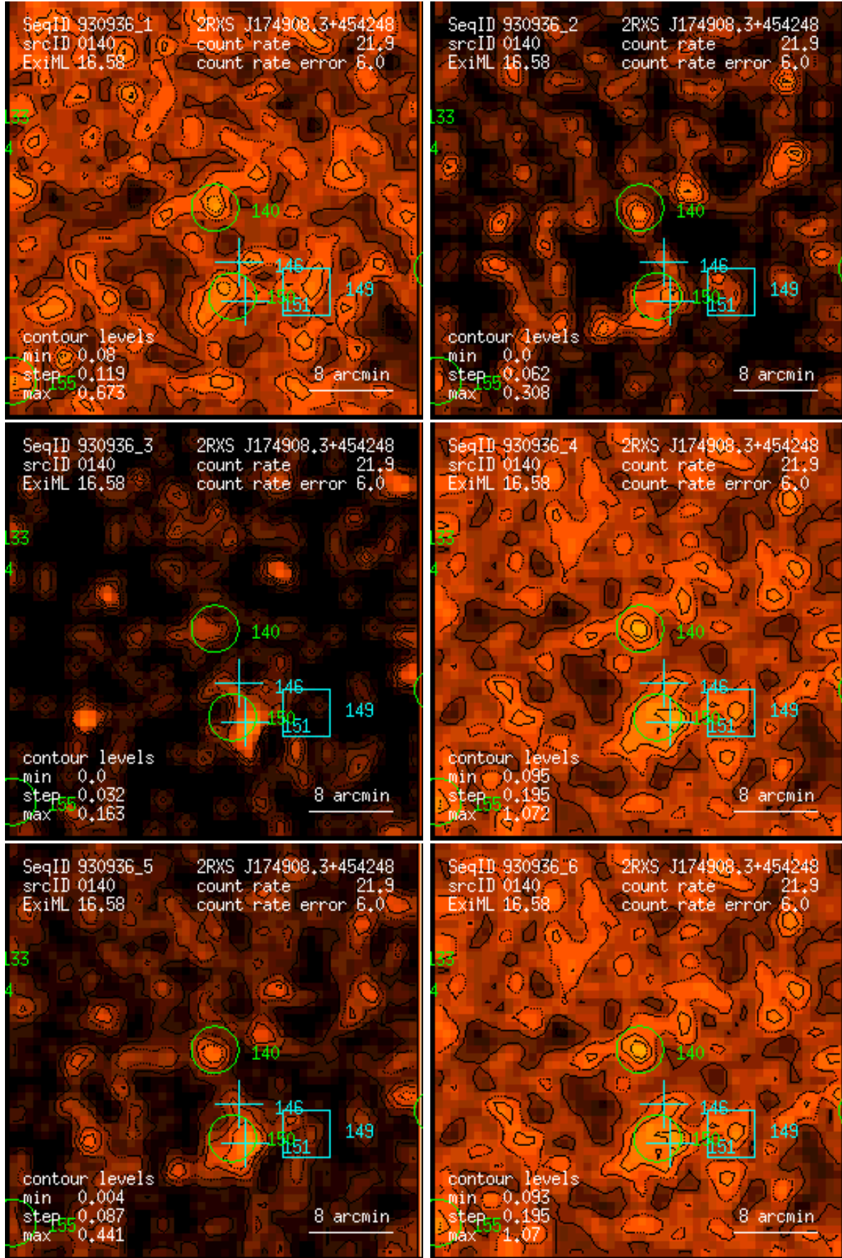
Figure 140: RASS 930936: detection 0140: band rate images, Gaussian filter: (1) PSPC channels 11 – 41, (2) 52 – 90, (3) 91 – 201, (4) 11 – 235, (5) 52 – 201, (6) 11 – 201. Broad band rates in counts/ks. Band rate contour levels in counts/ks/arcmin 2 .
