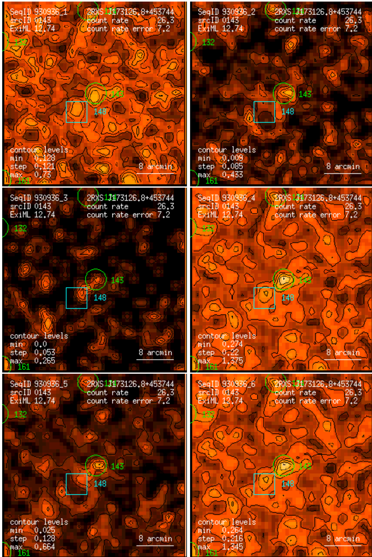
Figure 143: RASS 930936: detection 0143: band rate images, Gaussian filter: (1) PSPC channels 11 – 41, (2) 52 – 90, (3) 91 – 201, (4) 11 – 235, (5) 52 – 201, (6) 11 – 201. Broad band rates in counts/ks. Band rate contour levels in counts/ks/arcmin 2 .
